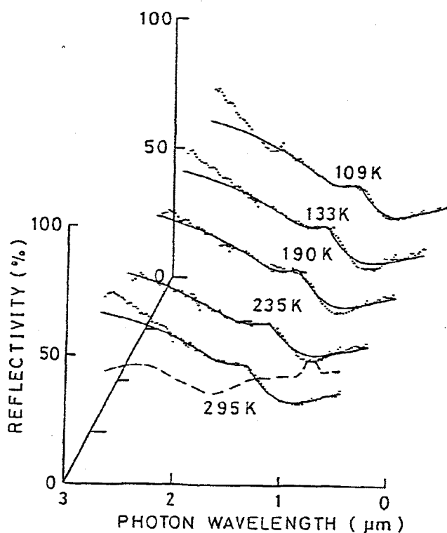
Fig. 2 Reflectivity of monoclinic \text{NbSe}_3 . Dotted lines show the experimental results for parallel polarization. Broken line shows for perpendicular polarization. Solid lines show the best fit for the experimental results using Eq. (2).
