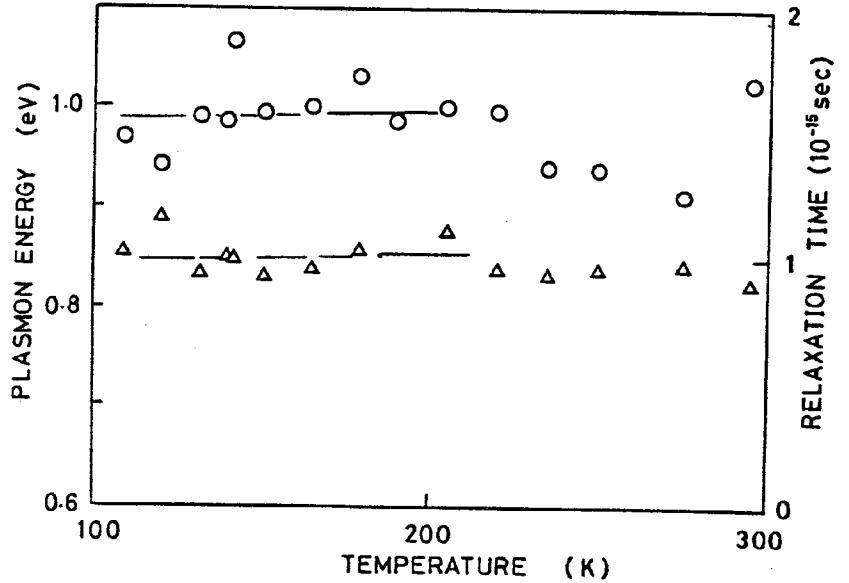
Fig. 7 Temperature dependence of plasmon energy (open circles) and its relaxation time (triangles) determined from the best fit of NbSe 3 .
