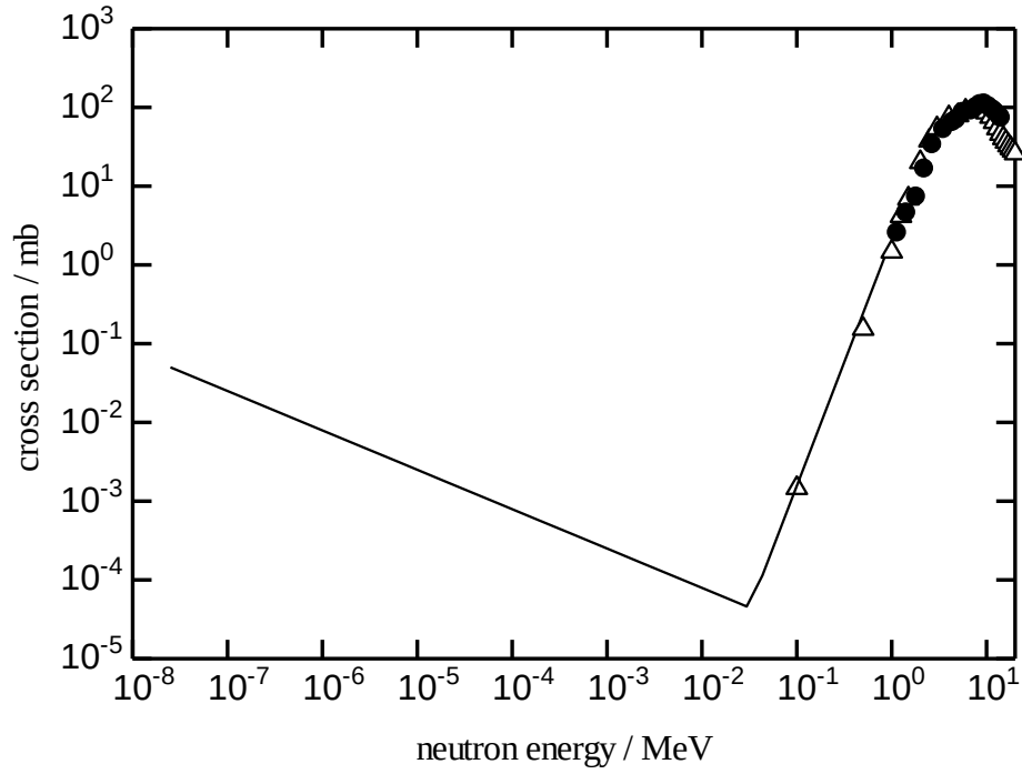
Fig. 1 Assumed excitation function of the reaction of ^{63}\text{Cu}(n, p)^{63}\text{Ni} (solid line) that was used in the recalculation of the number of ^{63}\text{Ni} nuclei produced in 1 g of copper. Circles and triangles show experimental cross section values (Takamiya et al. 2008b) and evaluated values from JENDL-3.3 (JENDL 2002), respectively.
