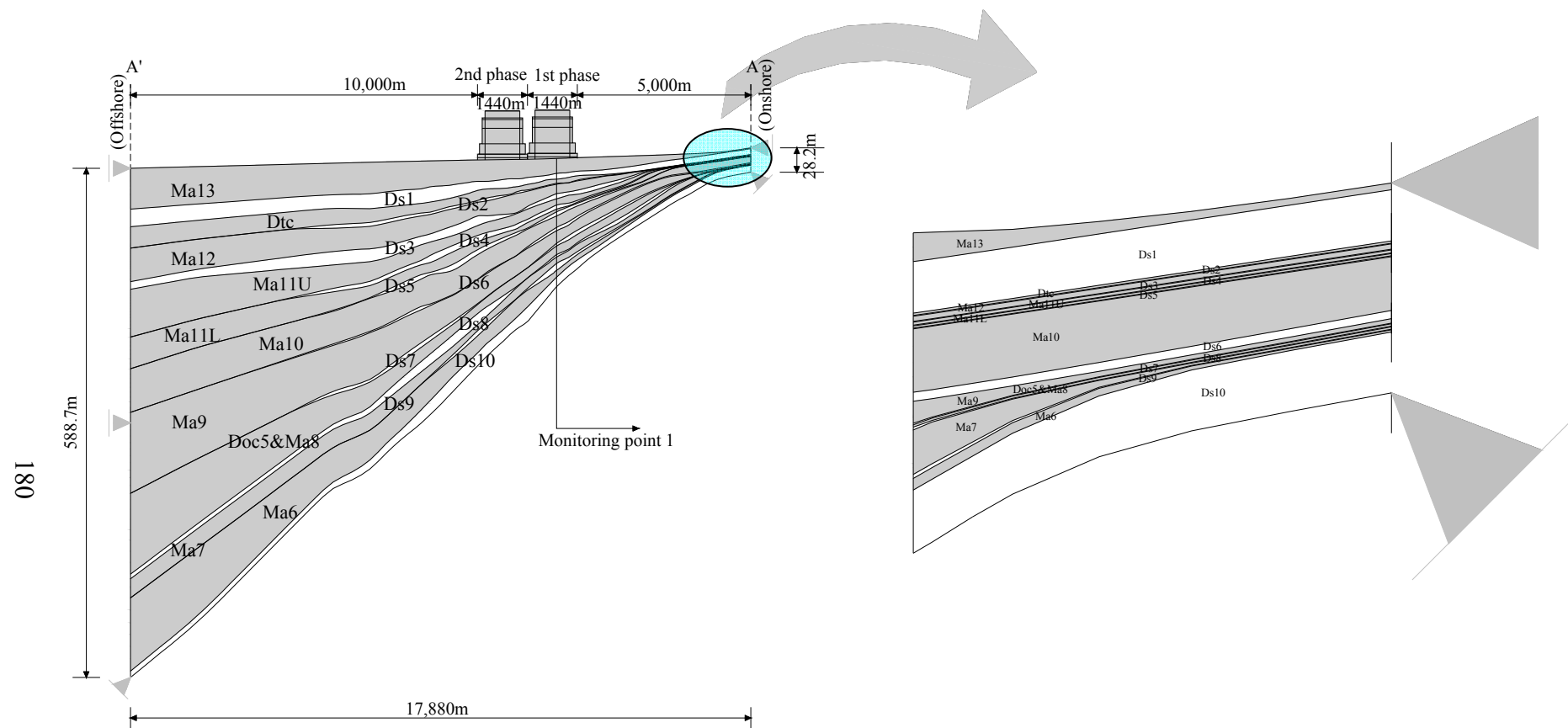
Fig. 6.10 Modified foundation model for the thickness of Ds10 layer near the boundary on the onshore side
