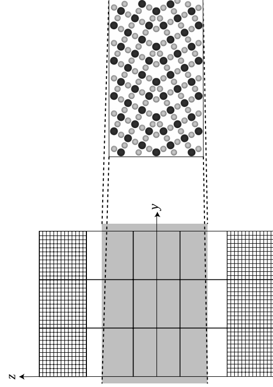
Figure 2.8 The model for molecular dynamics simulation for a grain-boundary structure in \text{Ni}_2\text{Y} phase. The schematic of the computational cell and the projected atomic arrangements. The periodic boundary conditions are posed on all borders except on the z borders. Meshed regions correspond fixed atoms.
