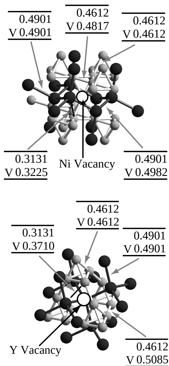
Figure B.1 Bond order change for the bondings near Ni and Y vacancy within second moment approximation. The values headed by 'V' are the bond order after vacancy formation.
