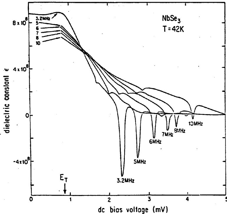
Fig. 16 Ac dielectric constant of NbSe 3 as a function of dc bias voltage. The dielectric constant is measured at various ac frequencies between 3 and 10 MHz. E_T is the threshold voltage for the onset of non-linear dc conduction.
