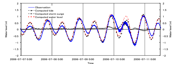
Fig. 12 The water level at Jeju of (b).
