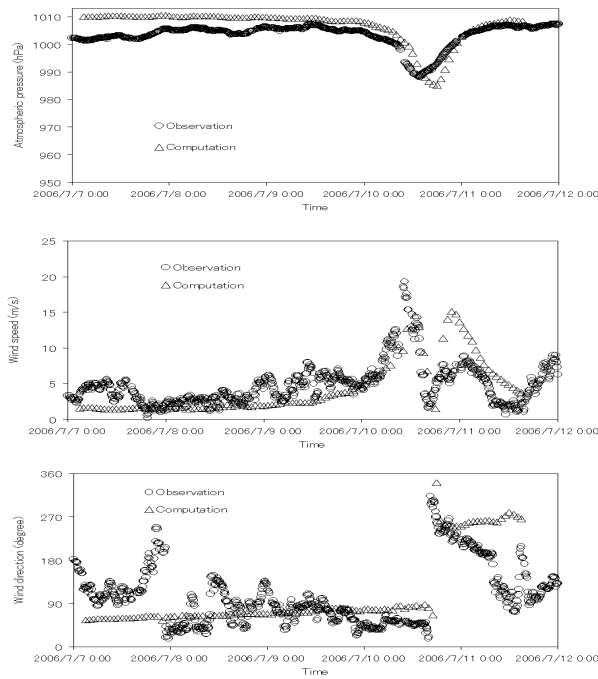
Fig. 7 The meteorological data observed at Sucheon of (3) (Upper; the atmospheric pressure, middle; the wind speed, lower; the wind direction).
