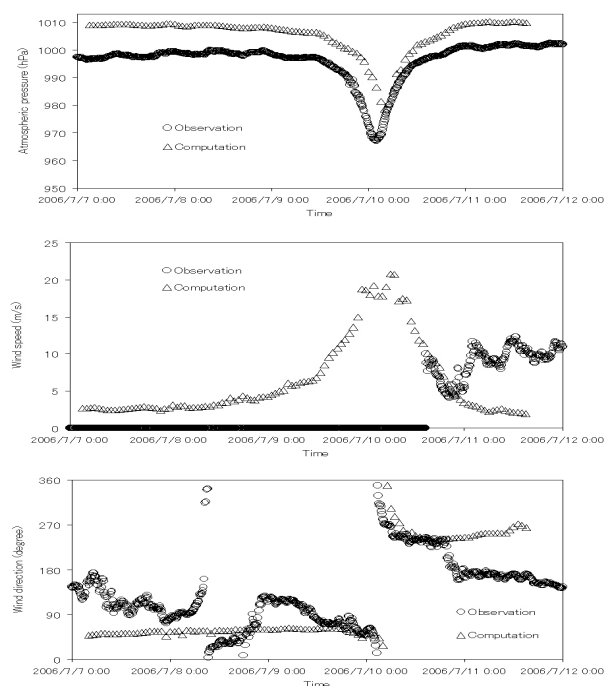
Fig. 5 The meteorological data observed at Iedo of (1) (Upper; the atmospheric pressure, middle; the wind speed, lower; the wind direction).
