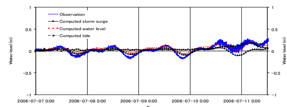
Fig. 15 The water level at Sokcho (d).
