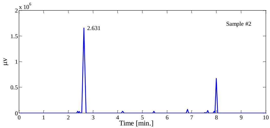
Figure 3.17 Chromatograph of rubber sample 2
