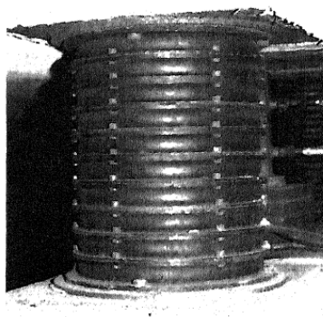
Figure 1.6 Steel rubber laminated bearing by Yokohama Rubber Co., 1969
