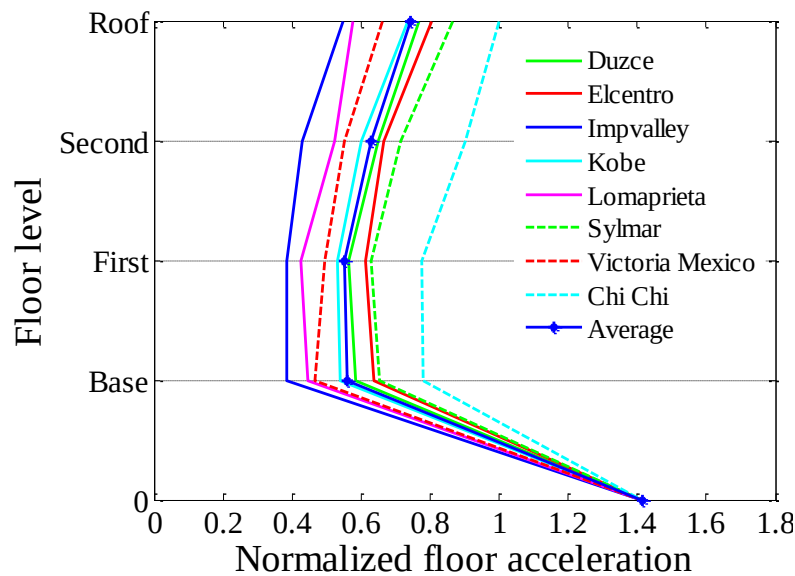
Figure 7.8 Normalized maximum absolute floor accelerations in x-direction for MCE
