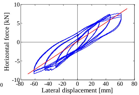
Figure 5.14 Load-displacement relationship
