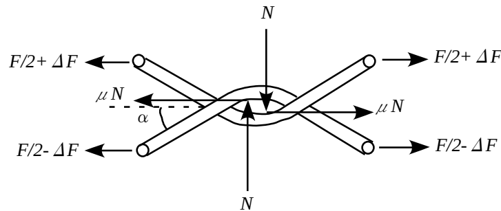
Fig. 4.21 Relative motion and friction forces
