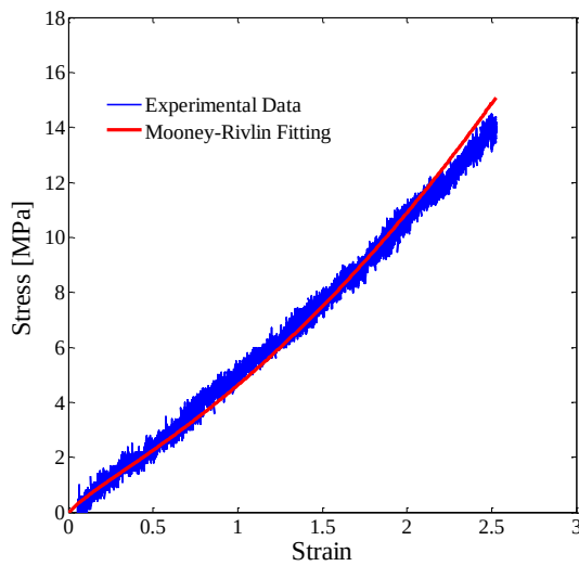
a) Monotonic tension test up to 50mm
