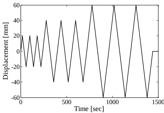
Figure 5.11 Input signal
