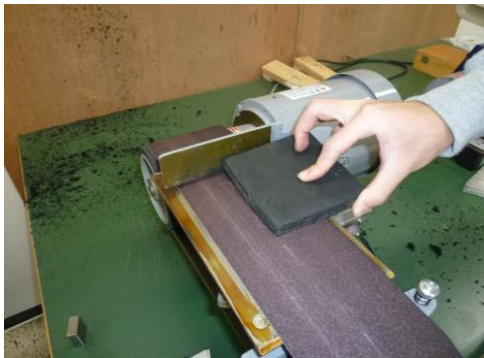
Figure 5.2 Sanding of layer is in progress
