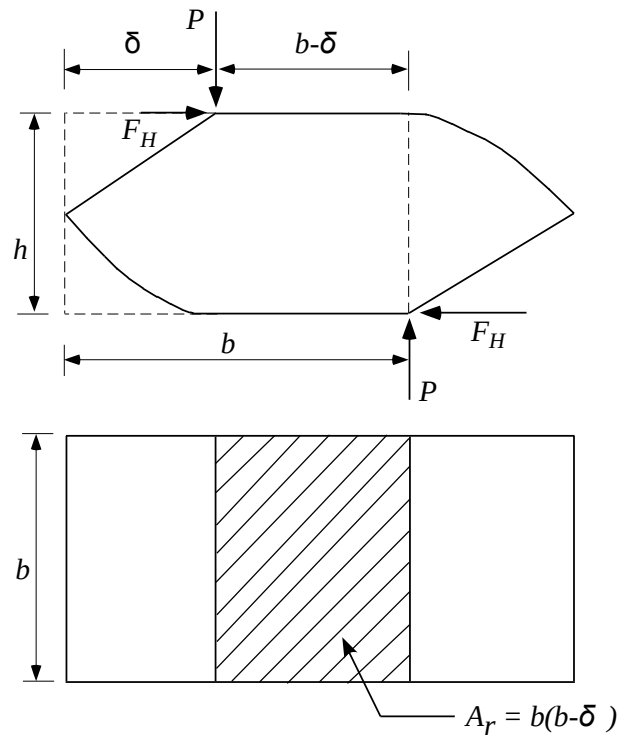
Figure 8.2 Deformed state of STRP bearing under combine loadings
