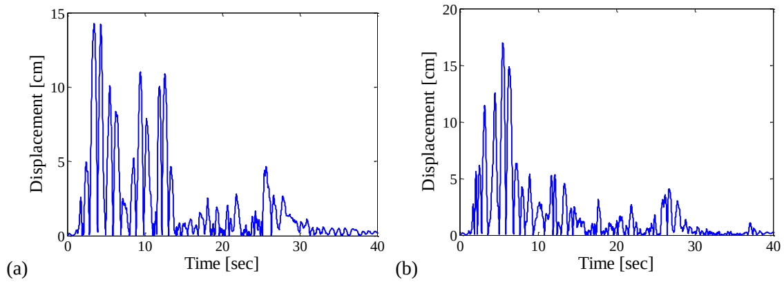
Figure 7.13 Absolute displacement plot at isolation floor a) x-direction b) y-direction due to El Centro record input for MCE
