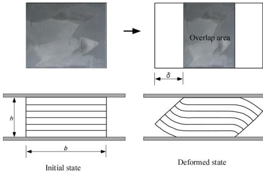
Figure 6.3 Lateral deformation pattern of layer-bonded STRP bearing
