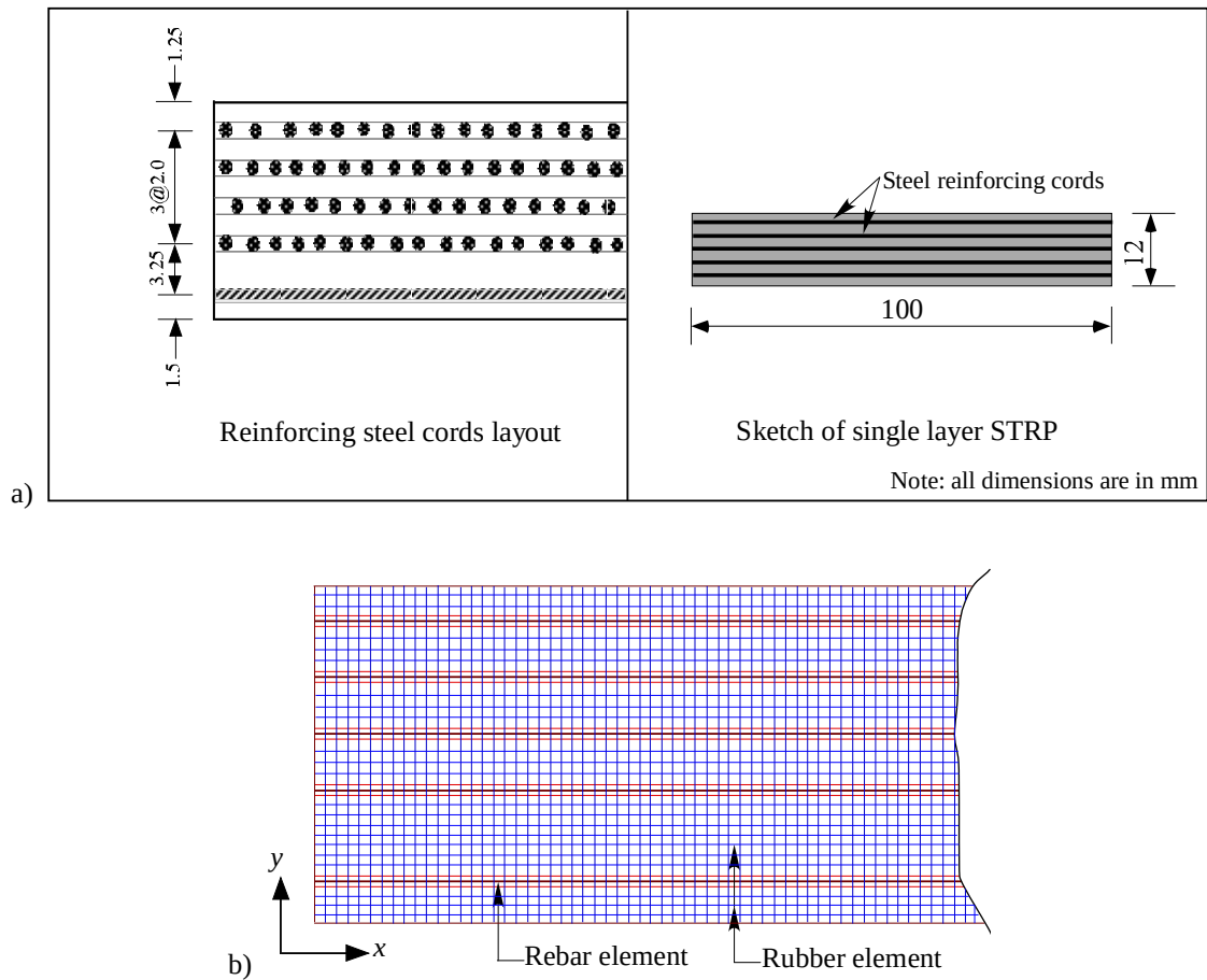
Figure 5.20 a) Dimensions and b) finite element mesh in a layer of STRP
