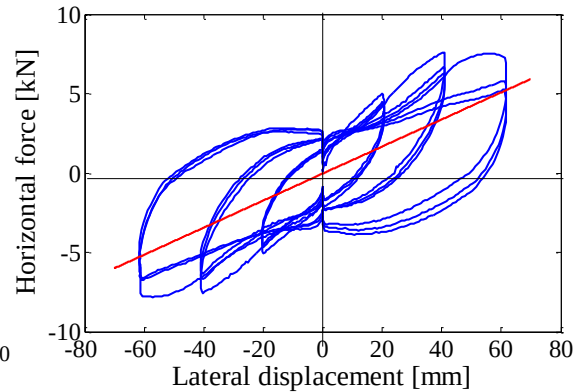
Figure 5.12 Load-displacement relationship
