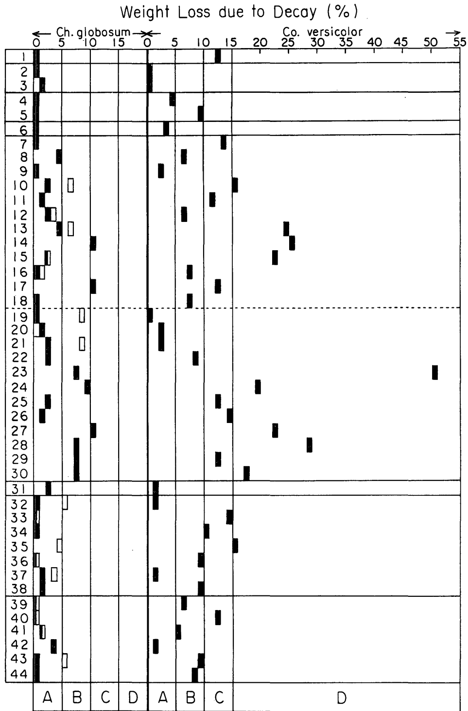
Fig. 2. Decay resistance of each softwood timber species against Ch. globosum and Co. versicolor .
