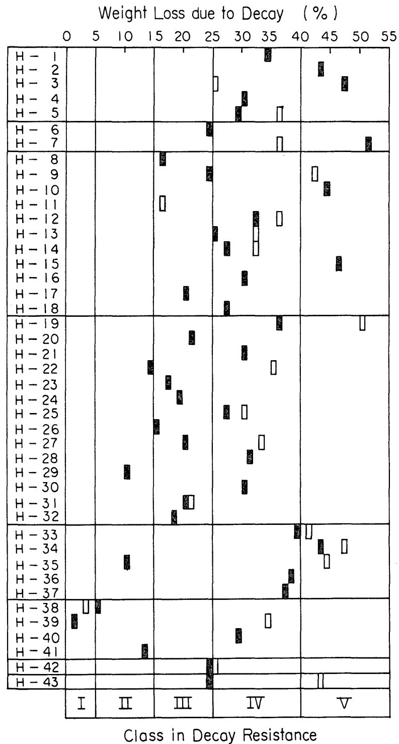
Fig. 1-1. Decay resistance of each hardwood timber species against Ch. globosum . Number at leftmost corresponds with the number of timber species shown in Table 1. Black and white rectangles are illustrated as the weight loss value in heartwood and sapwood samples, respectively.
