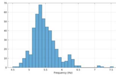
Figure 2. The histograms of the mathematical coefficients of bubble waveforms: (a) attenuation rate, (b) resonant frequency. The Y axes are event numbers.
