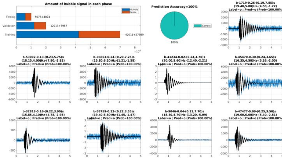
Figure 3. The examples of the synthetic waveforms (the black lines in each subplot). The varied noise levels are shown in blue.
