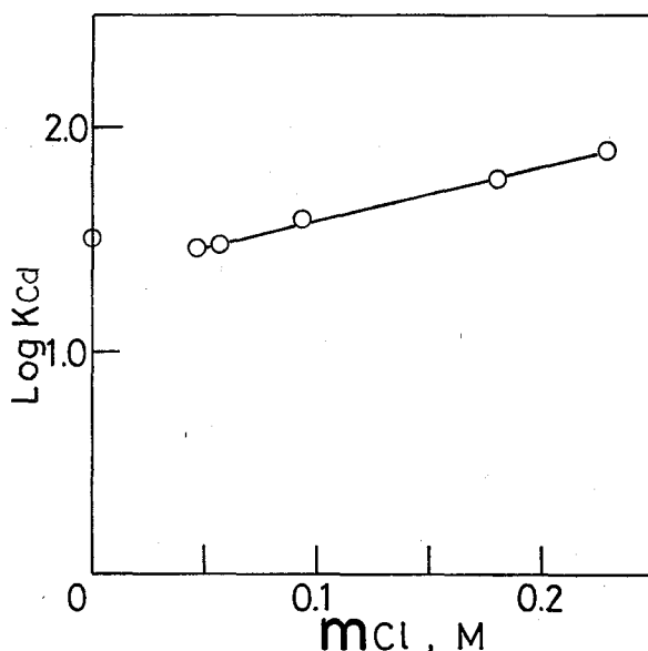
Fig. 5. The effect of chloride ions on the true distribution coefficient in magnesium chloride solution system.
