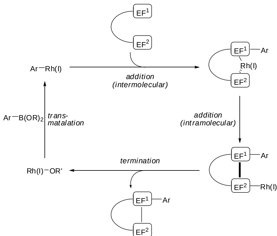
Figure 2. Concept of cascade cyclization triggered by addition of \text{Ar}-\text{Rh(I)}
