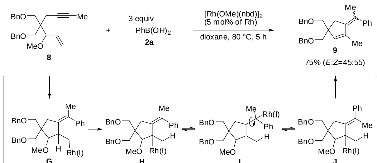
Scheme 2. Rhodium(I)-catalyzed arylative cyclization of 1,6-enyne 8 with phenylboronic acid
