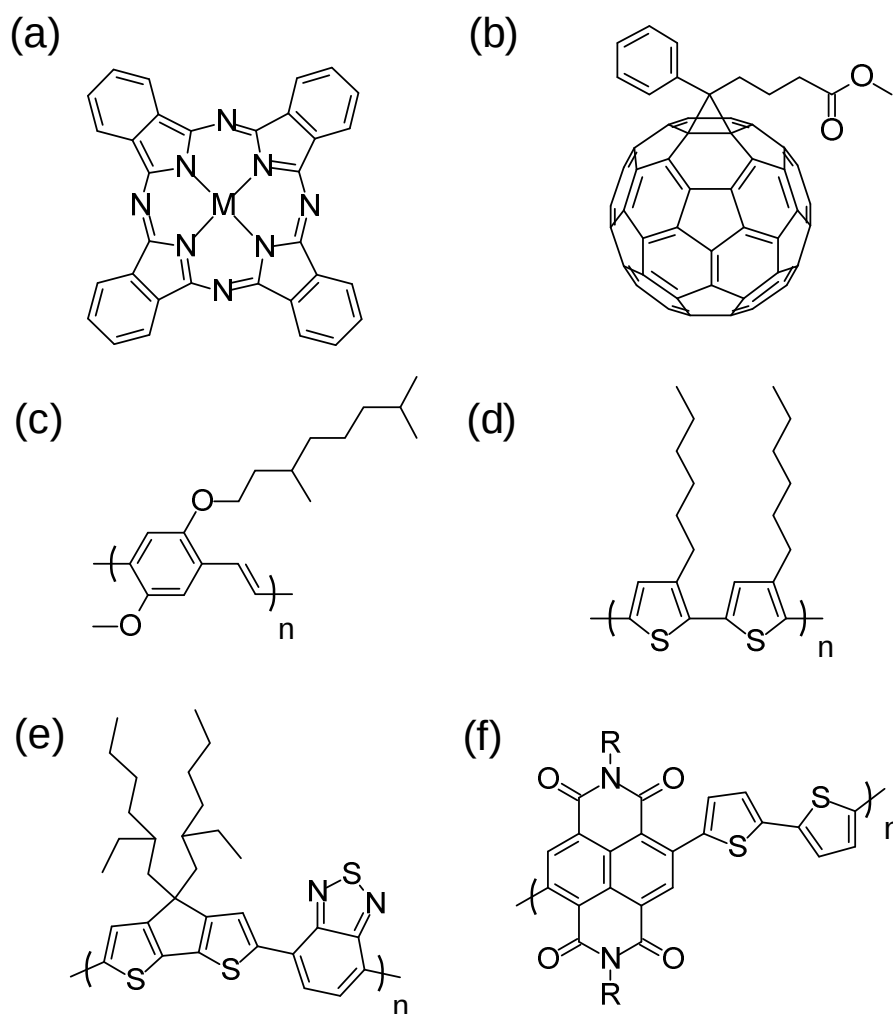
Figure 1-1. Chemical structures of representative organic semiconductors: (a) phthalocyanine (M = metal), (b) a fullerene derivative: [6,6]-phenyl-C 61 -butyric acid methyl ester (PCBM), (c) a poly( p -phenylenevinylene) derivative: poly[2-methoxy-5-(3,7-dimethyloctyloxy)-1,4-phenylenevinylene] (MDMO-PPV), (d) regioregular poly(3-hexylthiophene) (RR-P3HT), (e) a low-bandgap polymer poly[2,6-(4,4-bis-(2-ethylhexyl)-4 H -cyclopenta[2,1- b ;3,4- b' ]dithiophene)- alt -4,7-(2,1,3-benzothiadiazole)] (PCPDTBT) (f) a naphthalenediimide-based acceptor polymer poly{[ N,N' -bis(2-octyldodecyl)-naphthalene-1,4,5,8-bis(dicarboximide)-2,6-diyl]- alt -5,5'-(2,2'-bithiophene)} (P(NDI-2OD-T2)) (R = alkyl chain)
