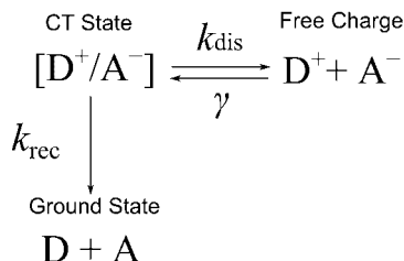
Scheme 5-1. Kinetic scheme for the bimolecular recombination via the CT state.
