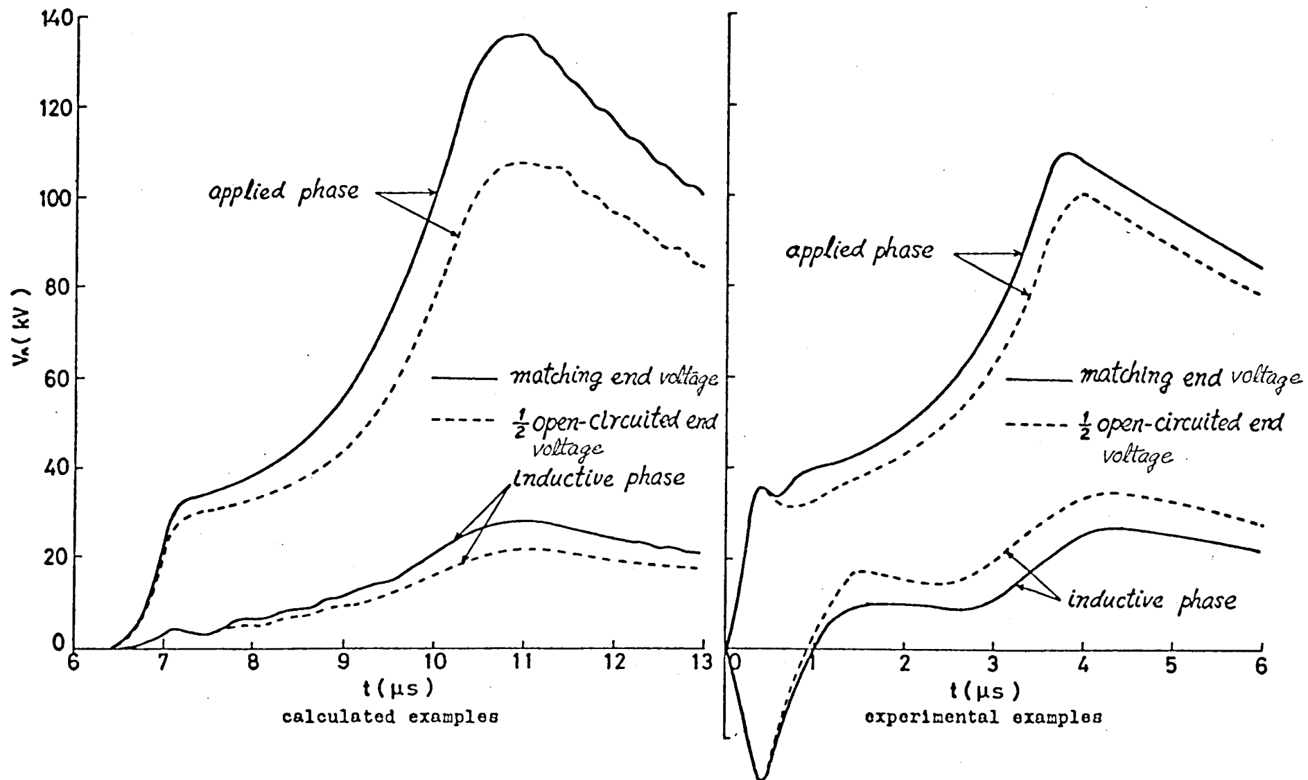
Fig. 6.5 Final end voltage waveforms when the impulse voltage ( E_0=230 \text{ kV} , \tau=5 \mu\text{s} ) is applied to one conductor and the other one is floated.
