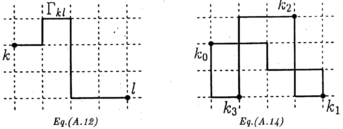
Figure 22: Gauge-invariant quantities.
