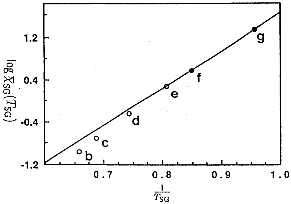
Figure 16: The data points b - g are fitted to the function
