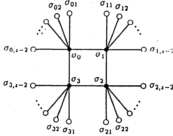
Figure 9: The cluster used in the "square approximation".
