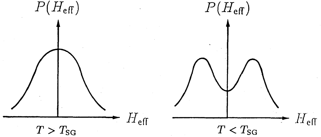
Figure 2: Schematic forms of the probability distribution of H_{\text{eff}} .
