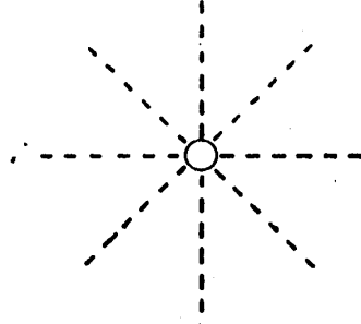
Figure 8: The “Weiss approximation”, or the Sherrington-Kirkpatrick model.
