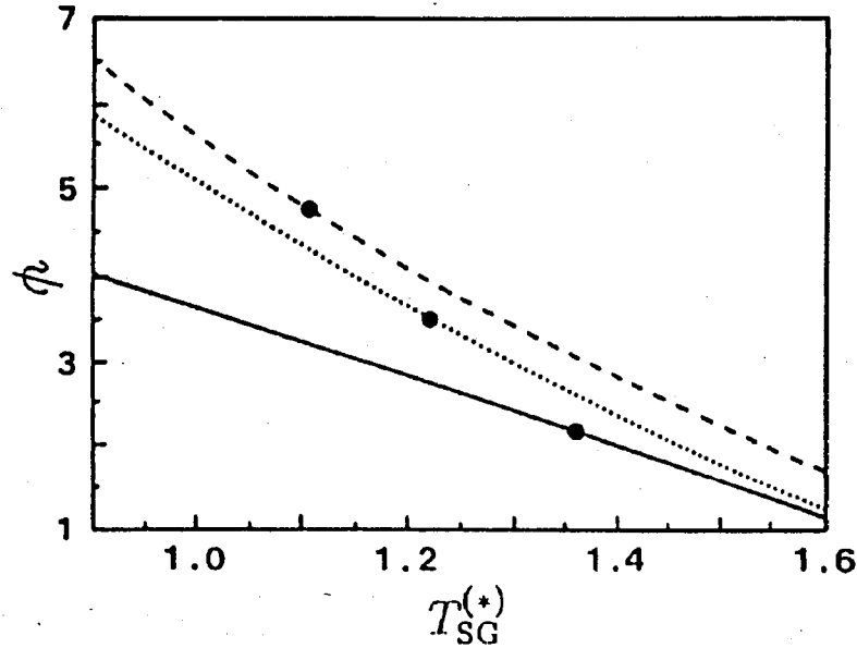
Figure 20: The values \psi fitted under the fixed values T_{SG}^{(*)} . Fitting variables are T_{SG} (the solid line), \tanh \frac{1}{T_{SG}} (the dotted line), and e^{-\frac{1}{T_{SG}}} (the broken line). The symbols “•” indicate the values of the best fittings.
