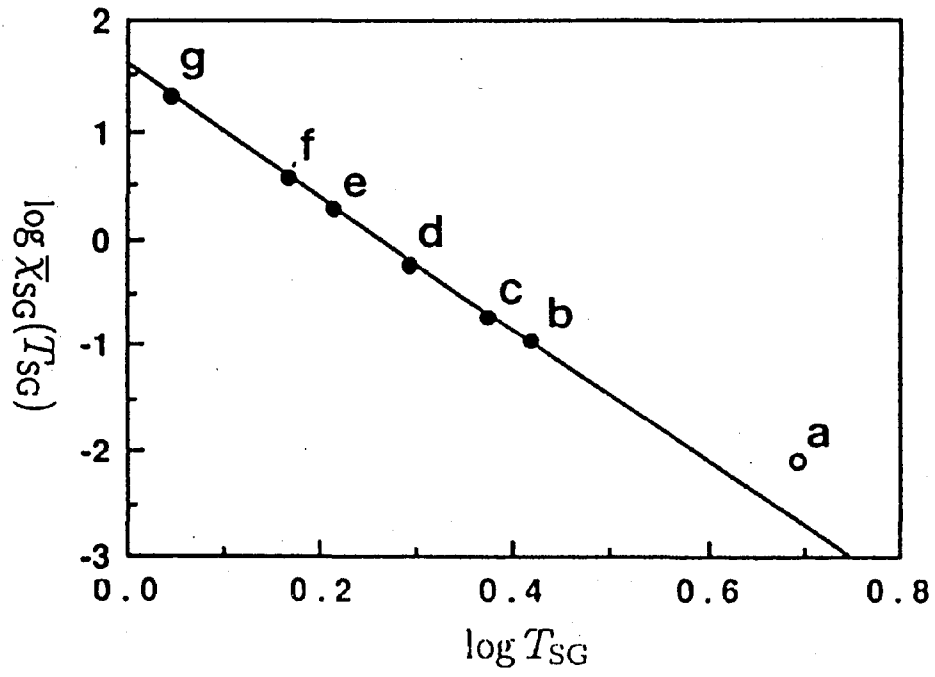
Figure 15: The data points b - g are fitted to the function
