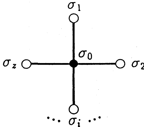
Figure 7: The cluster used in the “Bethe approximation”. The symbol “o” denotes the boundary sites, at which the effective fields are applied.
