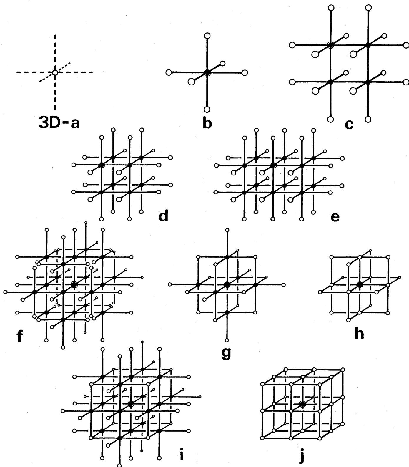
Figure 14: Treated clusters of the 3-dimensional system. The symbol "o" denotes the boundary sites of the clusters.
