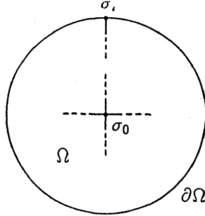
Figure 1: The cluster \Omega .
