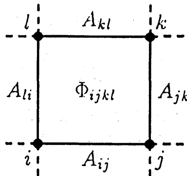
Figure 21: The definition of the frustration.
