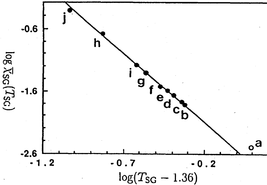
Figure 17: The data point b - g are fitted to the function
