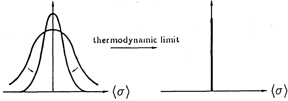
Figure 24: The fraction of the samples of \langle \sigma \rangle \neq 0 in the paramagnetic phase.
