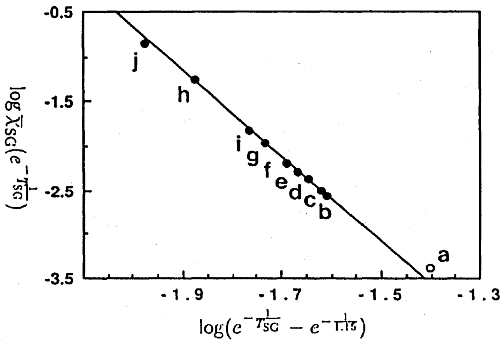
Figure 19: The data point b-g are fitted to the function
