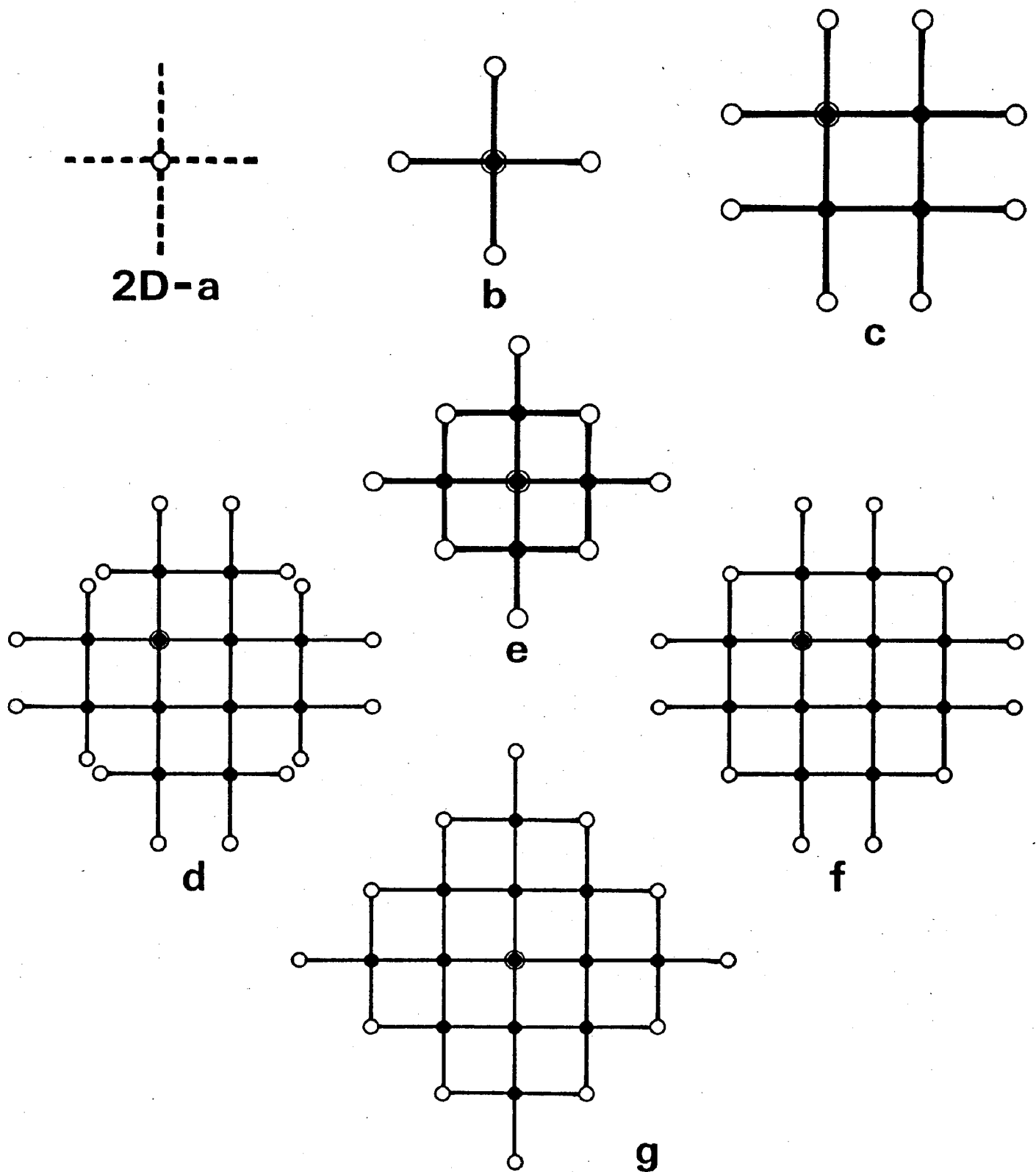
Figure 13: Treated clusters of the 2-dimensional system. The symbol "o" denotes the boundary sites of the clusters.
