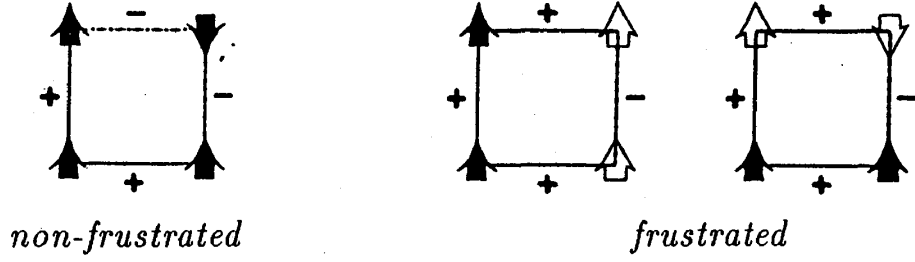
Figure 11: A non-frustrated plaquette and a frustrated one.
