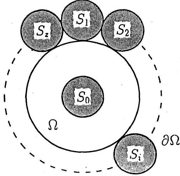
Figure 4: A cluster constructed of supports.
