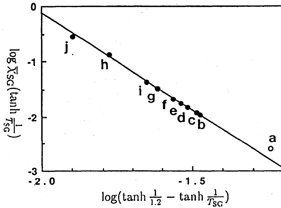
Figure 18: The data point b-g are fitted to the function
