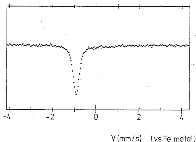
Fig. 2. Mössbauer spectrum of K_2Sr(FeO_4)_2 at room temperature
