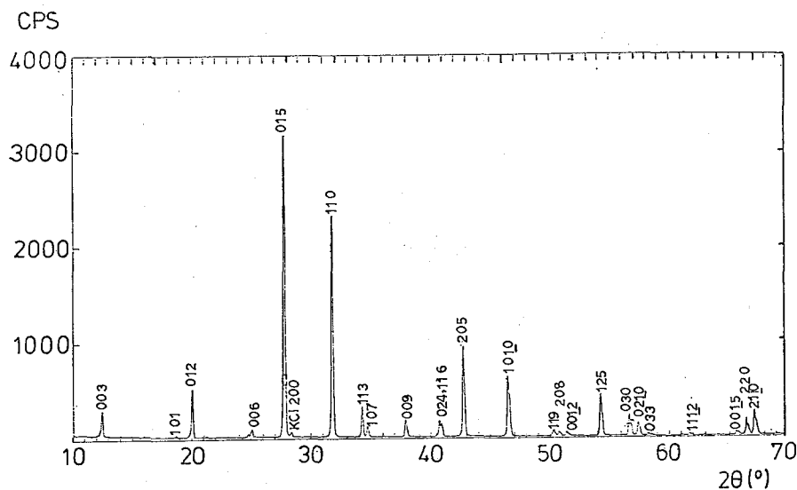
Fig. 1. X-ray diffraction pattern of \text{K}_2\text{Sr}(\text{FeO}_4)_2 .
