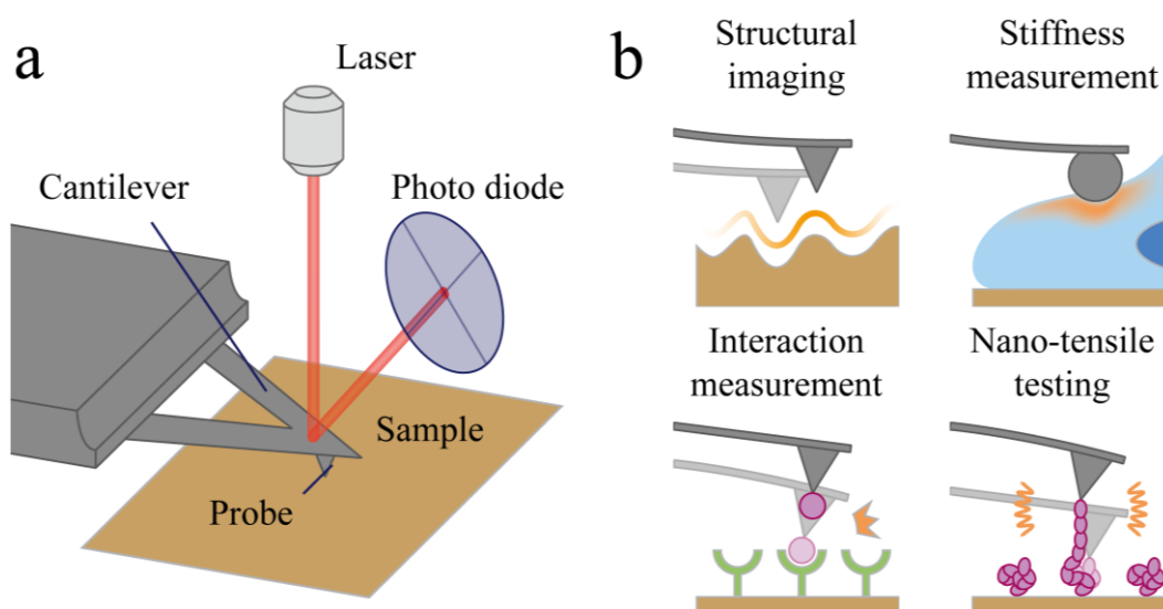
Figure 1-6: Principle of AFM and applications. a. An optical lever in AFM system. b. Structural imaging, stiffness measurement, interaction measurement, and nano-tensile testing.
