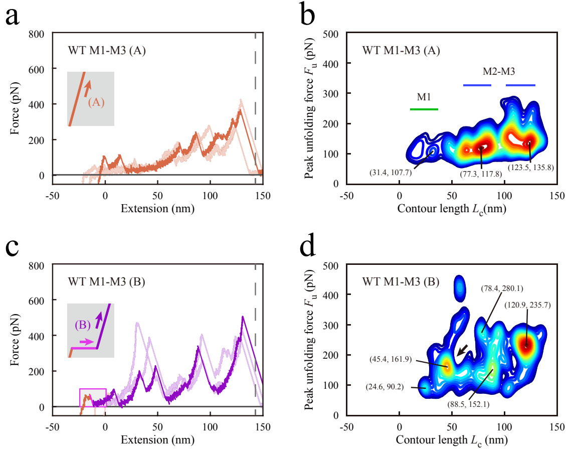
Figure 3-3: Results of AFM nano-tensile testing for WT M1-M3 domain in loading (A) and (B). a. Force curves for WT M1-M3 fragment in loading (A). The force curves are shifted to the left by the offset length L_{\text{offset}} . b. Contour map of number density n_d of force peaks in loading (A) based on 797 force curves. Color contours are set from the maximum value of n_d (red) to 0.4 \times the value (blue). c. Force curves in loading (B). d. Contour map in loading (B) based on 514 force curves.
