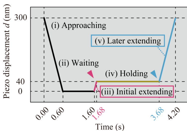
Figure 4-2: Programmed piezo displacement for AFM nano-tensile testing.
