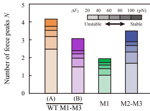
Figure 3-7: The average number of force peaks N per curve. The stacked bar graphs display N values, with color intensity illustrating the range of transition force \Delta F_T . The substructure stability increases with the increasing \Delta F_T values.
