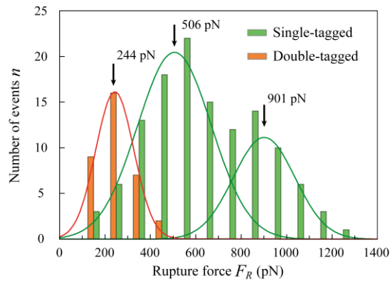
Figure 2-4: Histogram of F_R for single-tagged and double-tagged \beta -catenin.
