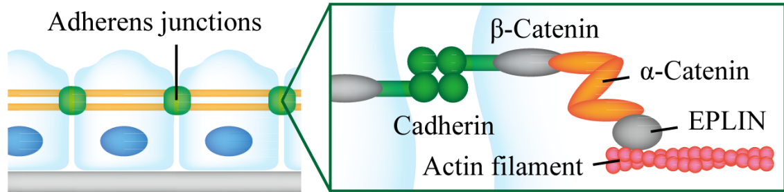
Figure 1-1: Cadherin-based adherens junctions. Several proteins such as \beta -catenin, \alpha -catenin, and EPLIN mediate the interaction between cadherin and actin filament.
