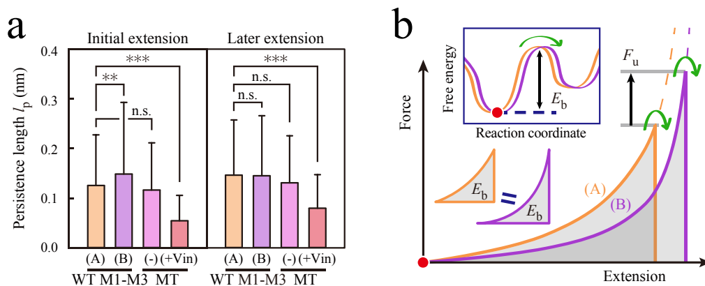
Figure 3-13: Persistence length analysis. a. Persistence lengths l_p . Error bars show standard deviations. Statistical significance in mean values was analyzed using t -test (**, p < 0.01 ; ***, p < 0.005 ). b. Effect of persistence length on peak unfolding force.
