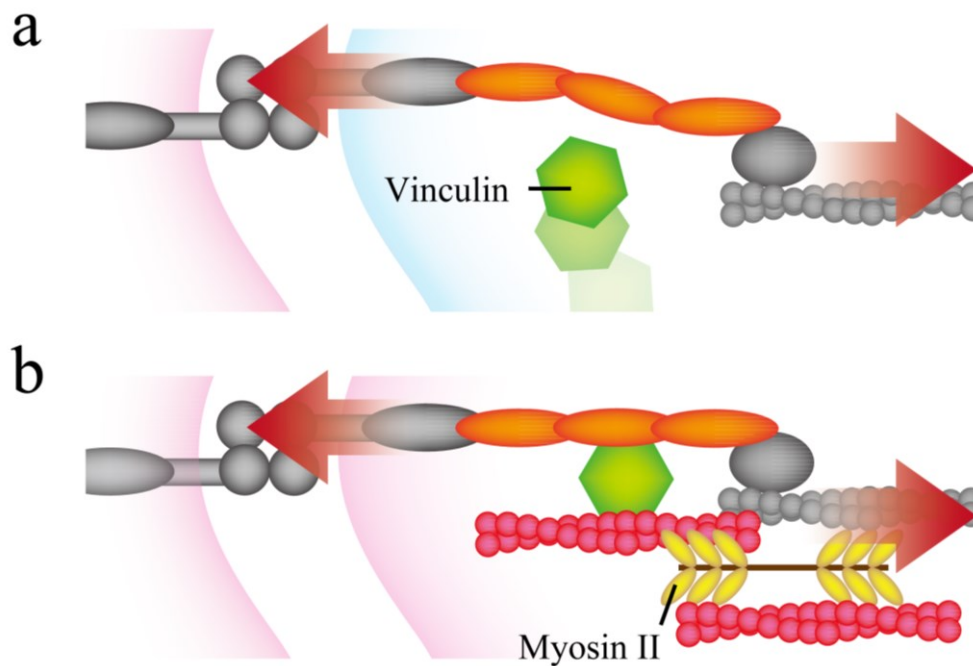
Figure 1-4: Molecular process of mechanotransduction at adherens junctions. a. The autoinhibition of \alpha -catenin is disrupted under intercellular tension resulting in vinculin association. b. Vinculin nucleates the actin remodeling, in which myosin II is involved in tension generation.
