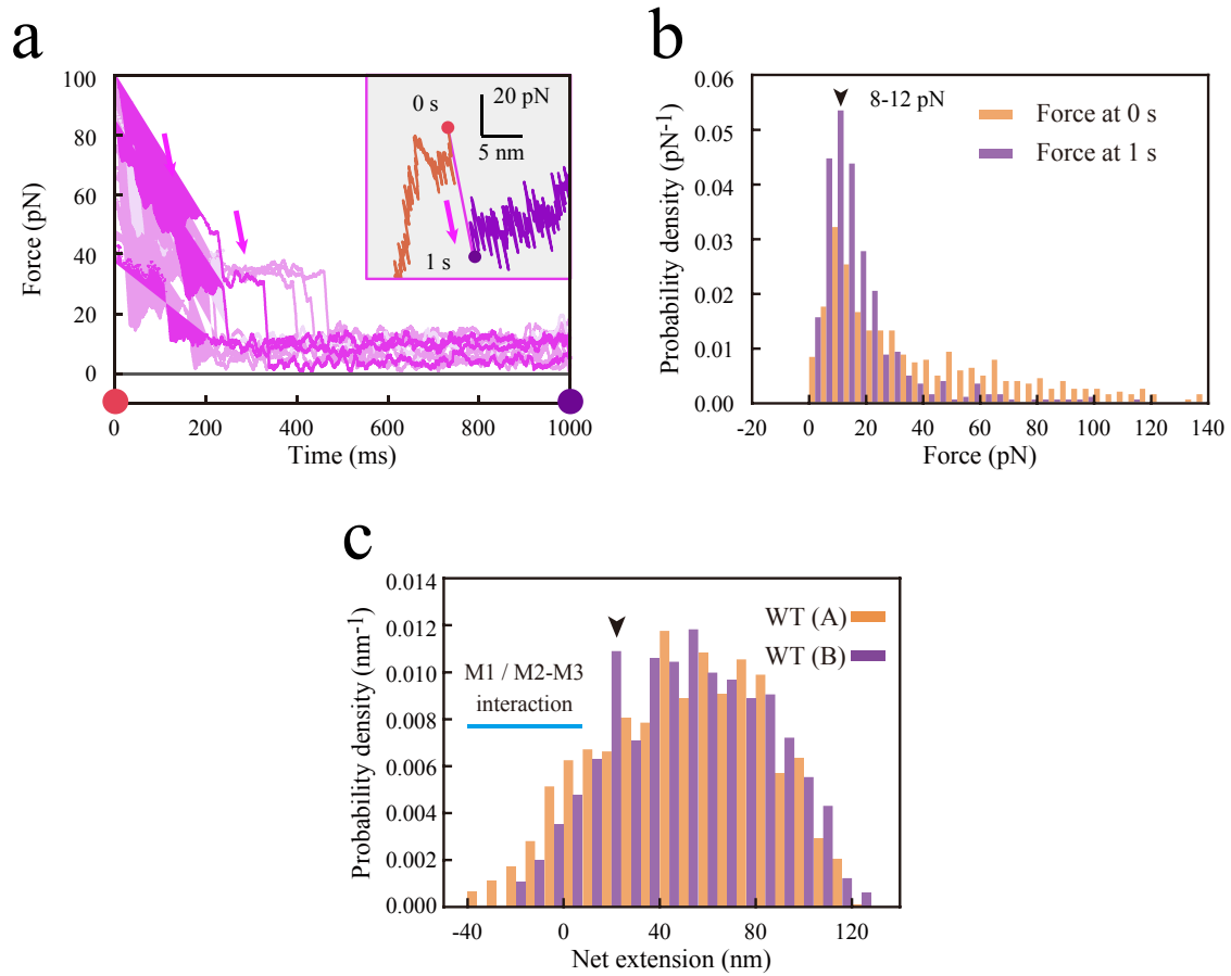
Figure 3-4: Conformational change in holding time. a. Force relaxation curve during the holding time. b. The probability density of force at 0 s (orange bars) and 1 s (purple bars) during the holding time. c. Histograms of the net extension of WT M1-M3 in loading (A) (orange bars) and loading (B) (purple bars). The arrowhead shows the salient peak in loading (B) corresponding to the peak indicated in the contour map. In the initial extension, the probability density in loading (B) was lower than that in loading (A), indicating that the M1/M2-M3 interaction was partly diminished during the holding time in loading (B).
