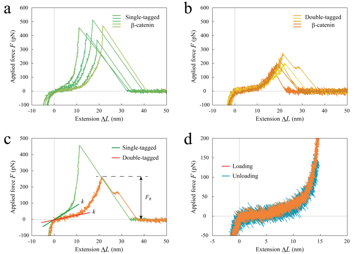
Figure 2-3: Results of AFM nano-tensile testing for \beta -catenin. a and b. Force curves for single-tagged ( a , green line) and double-tagged ( b , orange line) \beta -catenin. c. The rupture force F_R and initial spring constant k were analyzed. The orange and green linear lines indicate the linear regression curves in initial linear regions. d. Force curve obtained in loading (orange) and unloading (blue) double-tagged \beta -catenin experiments.
