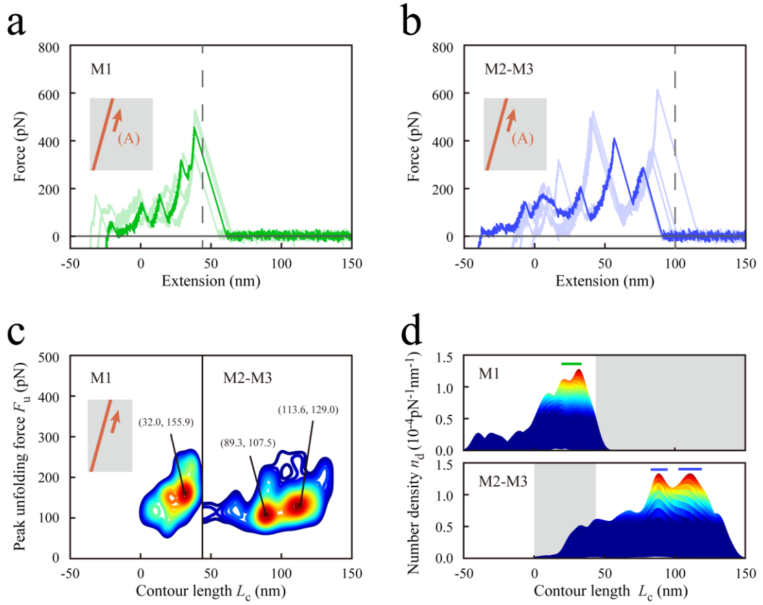
Figure 3-6: Results for segmented M1 and M2-M3 fragments. a and b. Force curves. c. Contour maps for M1 and M2-M3 fragments based on 181 and 785 force curves, respectively. The contour map for M2-M3 fragment is shifted to the right by 46.8 nm, which corresponds to the fully-extended length of M1 domain. d. Comparison of the number density n_d in contour maps against contour length L_c from a side view.
