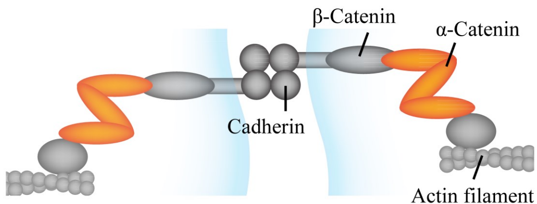
Figure 1-3: The molecular composition of adherens junctions. Cells are directly connected via cadherin, a transmembrane protein. \alpha -Catenin, connecting \beta -catenin and actin filament, forms an autoinhibited structure against vinculin in free condition.
