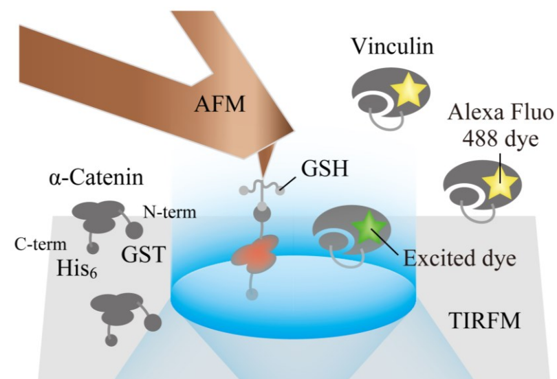
Figure 4-1: Schematic of an experiment using TIRFM-combined AFM. \alpha -Catenin molecules on coverslips were mechanically activated by AFM; simultaneously, full-length vinculin molecules in solvent were observed by TIRFM. Vinculin molecules were illuminated when they appear in an evanescent field (cyan region).
