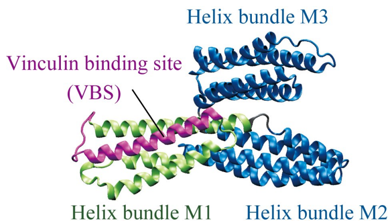
Figure 1-5: The crystal structure of tension-sensory domain \alpha -catenin (residues 277-631) [PDB code: 4K1N] (Ishiyama et al. 2013).
