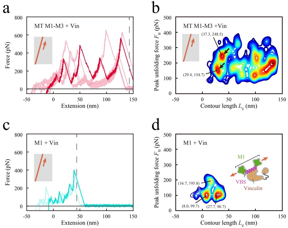
Figure 3-11: Effects of vinculin association on mechanical behaviors. a and c. Force curves for MT M1-M3 and M1 fragments associated with full-length vinculin. b and d. Contour maps MT M1-M3 and M1 fragments associated with full-length vinculin based on 571 and 111 force curves, respectively.
