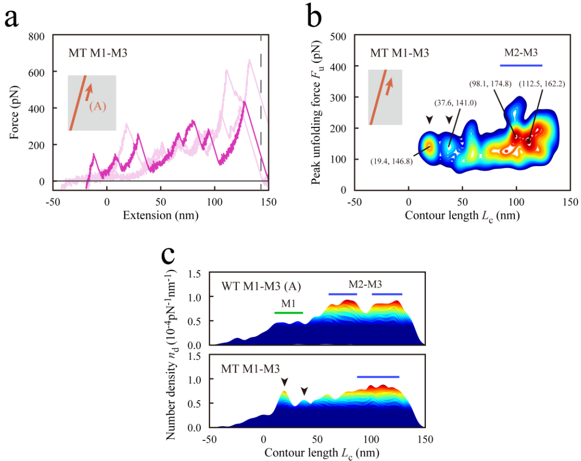
Figure 3-5: Results of nano-tensile testing for MT M1-M3 fragment. a. Force curves for MT M1-M3 domain. b. Contour map for MT M1-M3 fragment based on 576 force curves. c. Comparison of the number density n_d in contour maps from a side view in WT and MT M1-M3 fragments.
