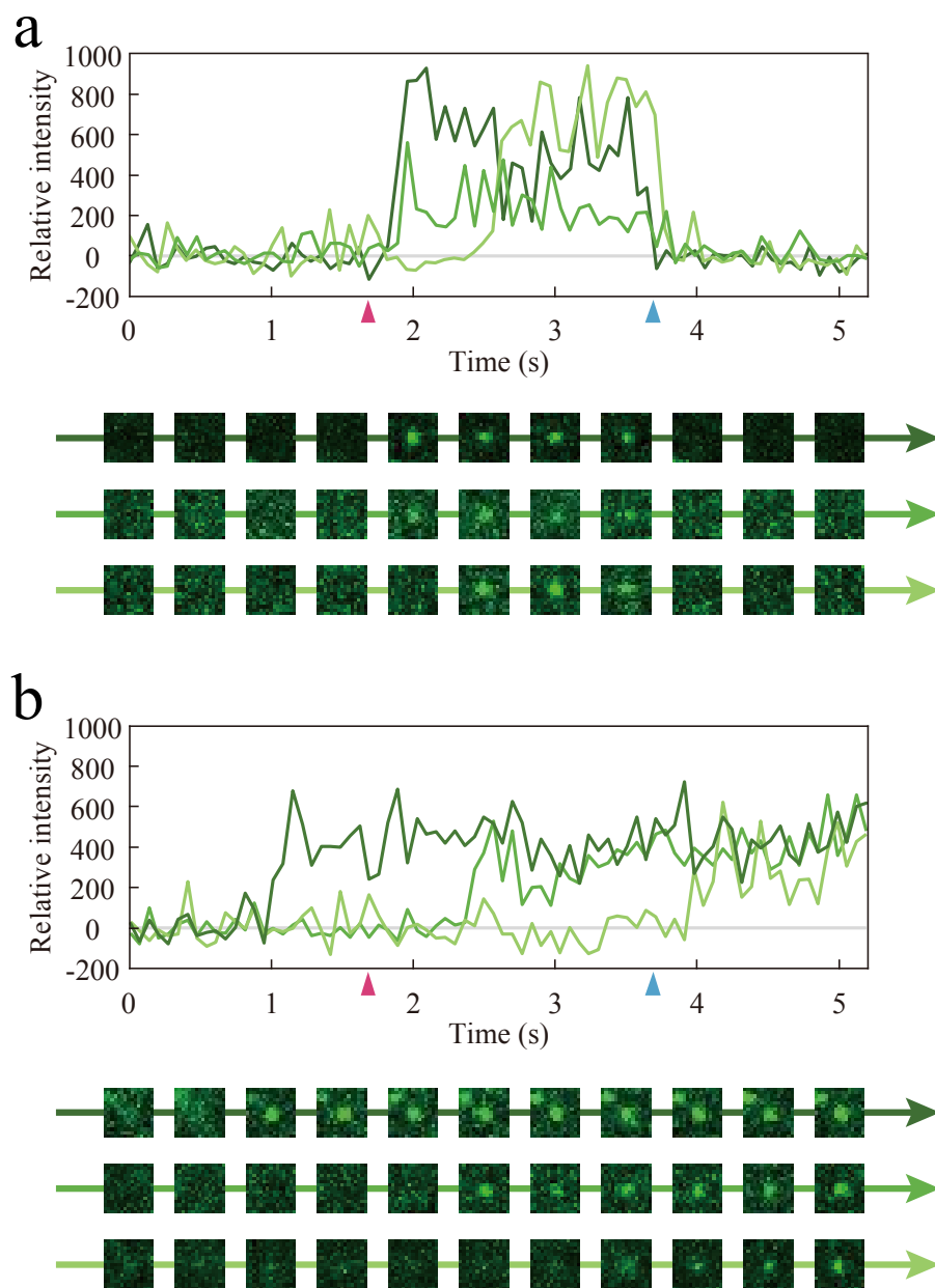
Figure 4-4: The results of TIRFM observation. a. Square pulses with increase in intensity after 1.68 s (magenta arrow head), representing vinculin association with mechanically activated \alpha -catenin and decrease at 3.68 s (cyan arrow head), representing vinculin dissociation caused by further \alpha -catenin extension. Time courses of images are shown in the lower panel. b. Step increases in intensity, independent of the timing of nano-tensile testing, caused by vinculin interaction with the surface of coverslip.
