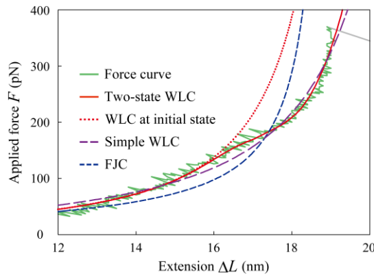
Figure 2-5: Results of curve fittings. Force curves (green line) were fitted by the two-state WLC model (red solid line), simple WLC model (purple long-dashed line), and FJC model (blue short-dashed line). The WLC curve at the initial state (red dotted line) was estimated from the result of fitting by the two-state WLC model.
