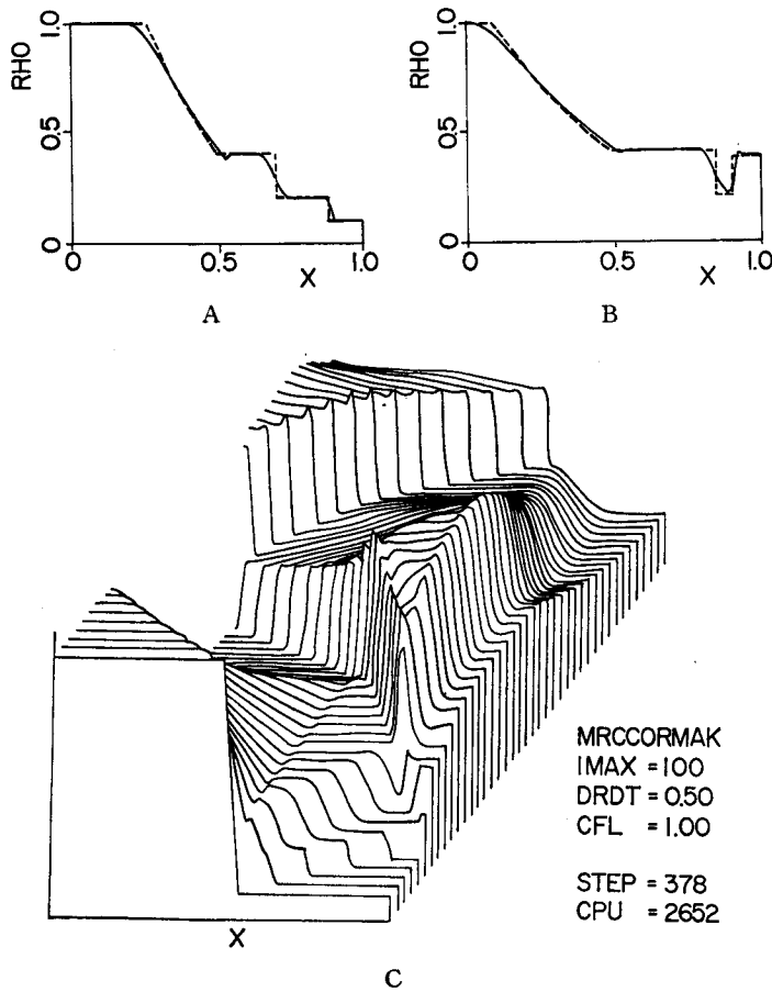
Fig. 2. Results for shock tube problem by the MacCormack method, the upper are the snap shots of density profile at t=0.2 and t=0.35 , and the lower snap shots show the time evolution of the density profile from t=0.0 to t=2.0 . IMAX means a number of meshes employed, DRDT the allowed maximum variation of density at one time step, CFL CFL number, STEP a number of steps used, CPU a computer processing time consumed.
