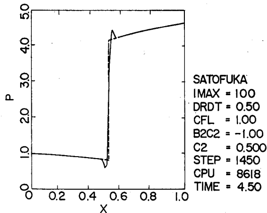
Fig. 9. Result by the Satofuka method. CFL number is 1.
