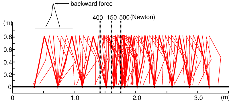
Figure 4. Stick figure of the walking motion adapting to successive perturbations (backward forces) affecting the hip joint. The dotted line denotes the position of the hip joint on the horizontal axis when each of the perturbations is applied. This motion is generated using the planned series of \phi_c values which is shown in Fig. 5. Re-establishing the leg posture at the BSP just after a perturbation enabled the walking system to overcome this series of strong perturbations.
