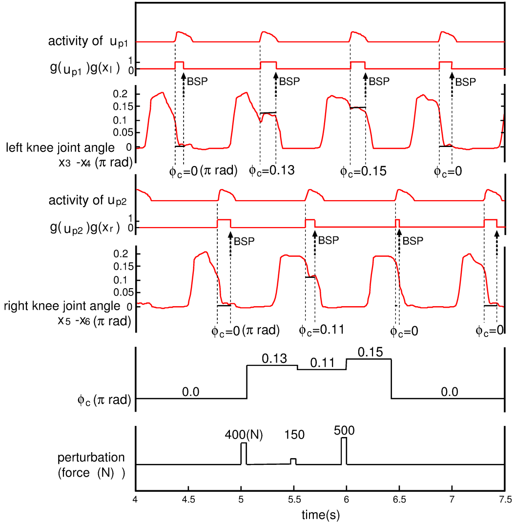
Figure 5. The motion of the knee joint angles around the period of successive perturbations. The series of equilibrium angles \phi_c prepared for the series of perturbations only works when the firing of the posture controller neuron falls during the swing phase, i.e. , when g(u_{p1})g(x_l) > 0 and g(u_{p2})g(x_r) > 0 (see (2.4)) for the left and right knees, respectively. At the BSP the knee joints are released from the equilibrium angle constraint \phi_c .
