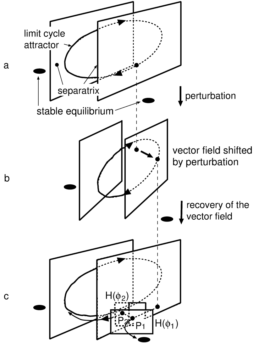
Figure 2. Schematic diagram showing the projection of the walking system's behavior in the phase space X onto the phase space \tilde{X} := \mathbf{R}^{35} . (a) A gait cycle and two falling states are translated into a limit cycle attractor and two stable equilibriums, respectively. (b) Schematic diagram illustrating the system motion when a perturbation affects the system ( 0.1s ). The perturbation is translated into a shift of the vector field. Because the attractor on the shifted vector field causes the system to approach it, the system motion deviates from the original limit cycle orbit. A large perturbation causes the system to cross over the original separatrix. (c) Schematic diagram illustrating reinitialization. Even if the system is strongly perturbed, the gait can be maintained. At a position P_1 occurring on the path the system takes while approaching a stable equilibrium, the posture controller causes the system state to be reset from P_1 to another position P_2 near the separatrix and on the side where the limit cycle exists. At P_2 , the system is immediately attracted to the limit cycle. The positions P_1 and P_2 are on the hyperplanes H(\phi_1) and H(\phi_2) , respectively.
