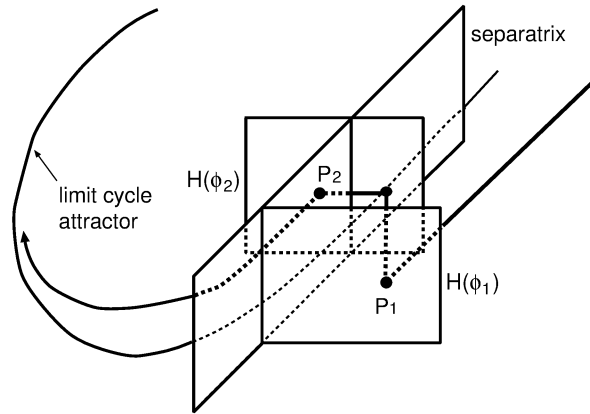
Figure 7. Schematic diagram illustrating the image in \tilde{X} of the reinitialization process which is considered to be reproduced exactly in simulations of the model. The shift of the moving point P(t) from P_1 to P_2 can be understood to embody the following two characteristics. 1) First the moving point P(t) arrives at H(\phi_2) in a very short time. Next, 2) the point P(t) moves along H(\phi_2) until it arrives at P_2 . Arriving at P_2 , the orbit immediately restarts from this position, obeying the dynamics of the coupled system. The orbit is then attracted by the limit cycle attractor.
