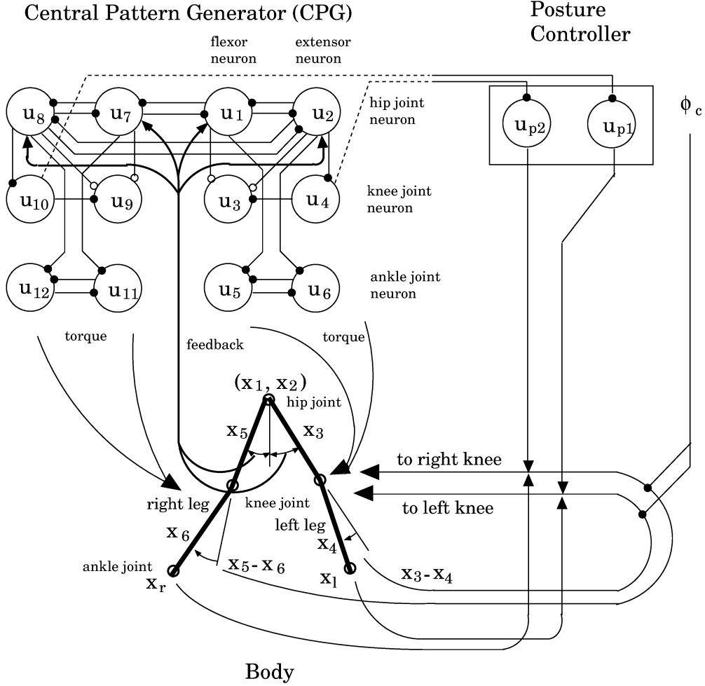
Figure 3. The walking system consists of the posture controller (neurons p1 to p2 ) and the coupled system composed of the central pattern generator (CPG) (neurons 1 to 12) and the body. \circ and \bullet denote excitatory and inhibitory Connections, respectively. The motion of the hip, the knee and the ankle in the left leg is governed by neurons 1 – 2, 3 – 4 – p1 and 5 – 6, respectively. Similarly, the motion of the joints in the left leg is governed by neurons 7 to 12 and p2 . Odd-numbered neurons and even-numbered neurons in the CPG controller represent flexors and extensors, respectively. The posture controller provides the equilibrium angle \phi_c for the knee joint at the BSP.
