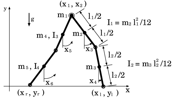
Figure 8. Model of a bipedal body as an interconnected chain of 5 rigid links (a point mass m_1 on the hip and 4 rigid bodies I_i (i = 1, 4) ).
