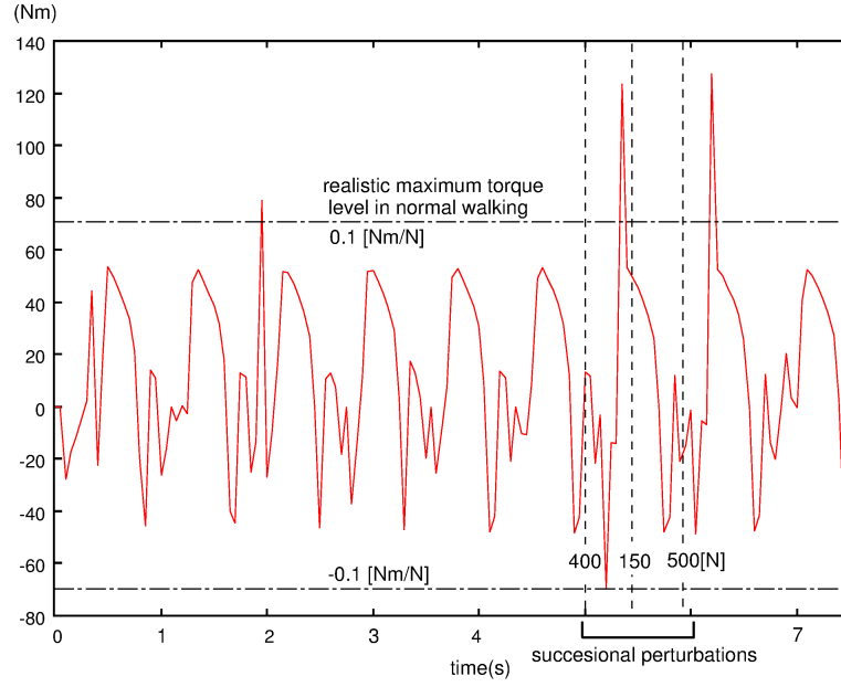
Figure 6. Sequential changes of the torque acting in the left knee joint ( T_{r2} in the appendix) in the case where the hip is perturbed by external forces. The dotted line denotes the times when perturbations are applied.
