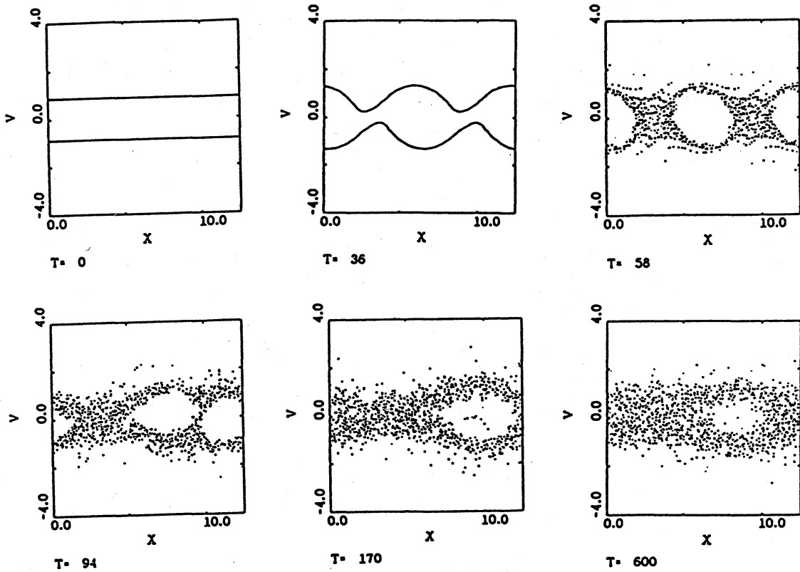
Fig. A typical evolution of 1260 sheets in the phase space.
