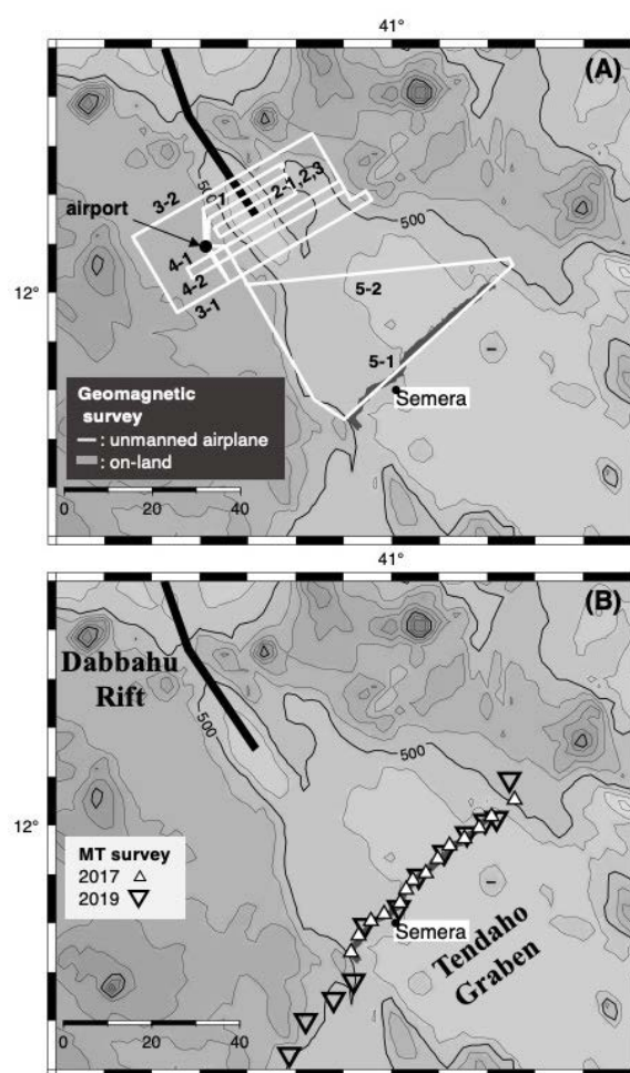
Fig.2. (A) Geomagnetic surveys. On-land geomagnetic surveys (gray line) and flight tracks of an unmanned airplane for aero-geomagnetic survey (white lines). (B) MT surveys.
