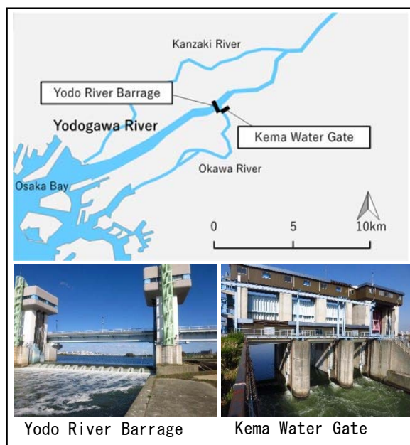
Fig. 4 Estuary of the Yodo River and survey point for larval drift of Ayu-fish
