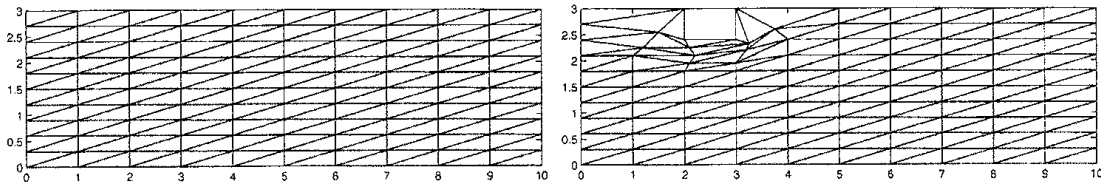
Figure 9: Friedrichs-Keller grids used for the simulation of pipe flow and pipe flow below a protruding step (inflow on the left, outflow on the right, i.e. open boundaries on the left and right end with a nonzero velocity gradient and fixed boundaries on top and bottom). The grid points around the step in the grid on the right were chosen to minimize the dislocation of the other grid points, not to minimize the error in the spacial discretization.
