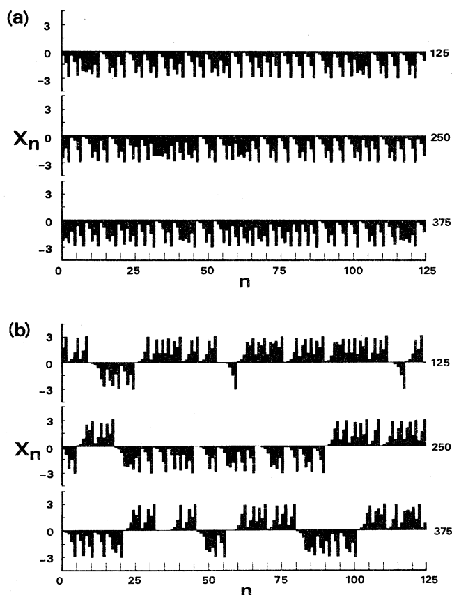
FIG. 3. Waveforms of Eq. (11) for (a) \mu = 3.11 (before the crisis) and (b) \mu = 3.17 (after the crisis). Bar graph of X_n as a function of n for 375 iterations after preiteration.
