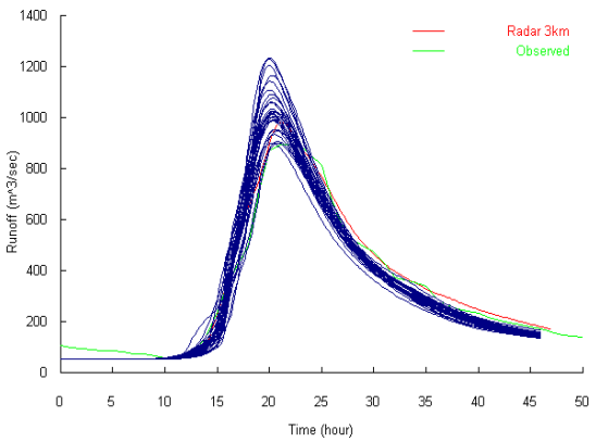
Fig. 14. Hydrographs at Kamo (1,469 km 2 ) obtained from the use of rainfall disaggregated by the RCHSA method
