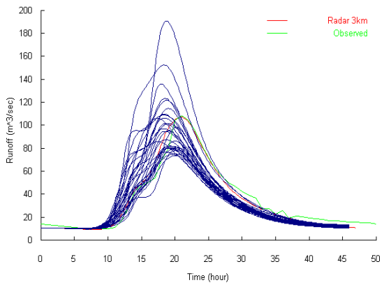
Fig. 20. Hydrographs at Ootori (156 km 2 ) obtained from the use of rainfall disaggregated by the RCHSA method
