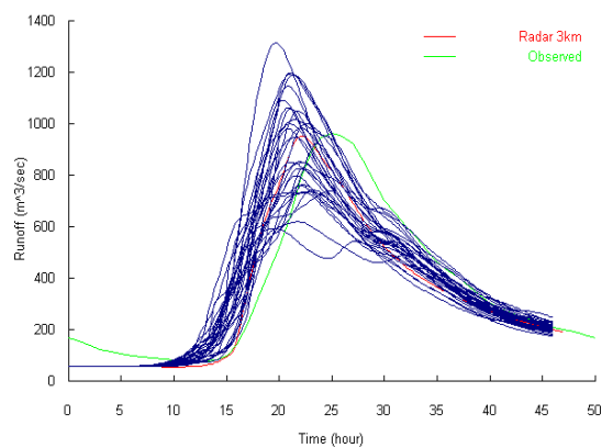
Fig. 10. Hydrographs at Inooka (1,589 km 2 ) obtained from the use of rainfall disaggregated by the RC method
