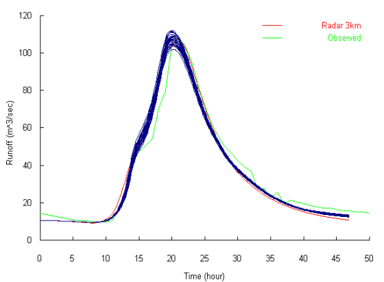
Fig. 21. Hydrographs at Ootori (156 km 2 ) obtained from the use of rainfall disaggregated by the STRaM method
