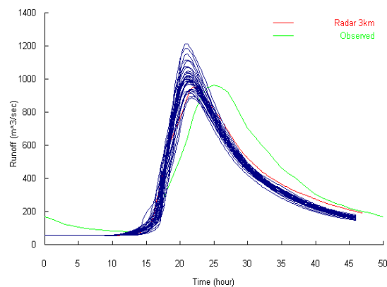
Fig. 11. Hydrographs at Inooka (1,589 km 2 ) obtained from the use of rainfall disaggregated by the RCHSA method
