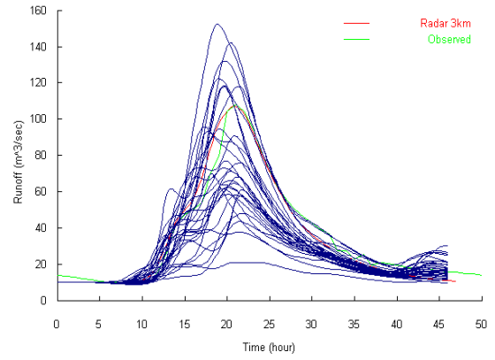
Fig. 19. Hydrographs at Ootori (156 km 2 ) obtained from the use of rainfall disaggregated by the RC method
