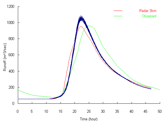
Fig. 12. Hydrographs at Inooka (1,589 km 2 ) obtained from the use of rainfall disaggregated by the STRaM method
