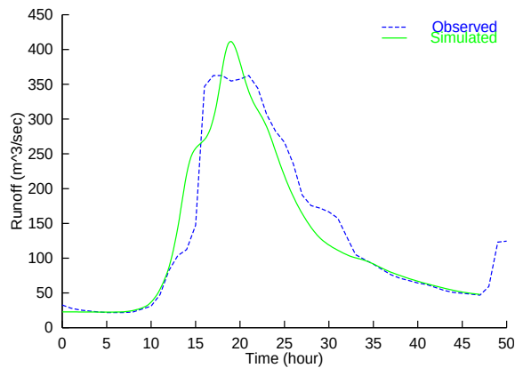
Fig. 8. Hydrograph at Ieno (476 km 2 )
