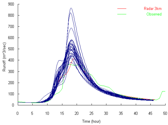
Fig. 17. Hydrographs at Ieno (476 km 2 ) obtained from the use of rainfall disaggregated by the RCHSA method
