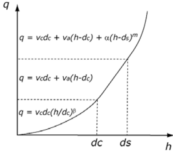
Fig. 3. Stage-discharge relationship for saturated-unsaturated layer
