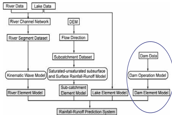
Fig. 4. Schematic of the Yodo River Model components
