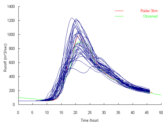
Fig. 13. Hydrographs at Kamo (1,469 km 2 ) obtained from the use of rainfall disaggregated by the RC method
