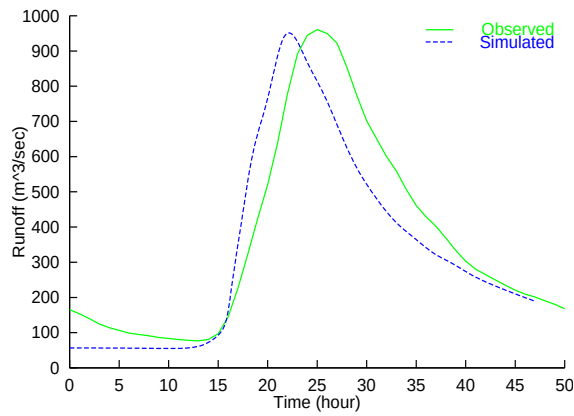
Fig. 6. Hydrograph at Inooka (1,589 km 2 )
