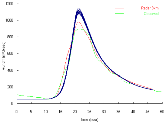
Fig. 15. Hydrographs at Kamo (1,469 km 2 ) obtained from the use of rainfall disaggregated by the STRaM method
