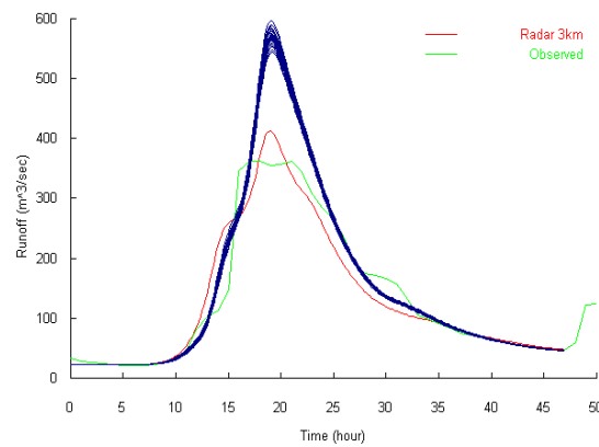
Fig. 18. Hydrographs at Ieno (476 km 2 ) obtained from the use of rainfall disaggregated by the STRaM method
