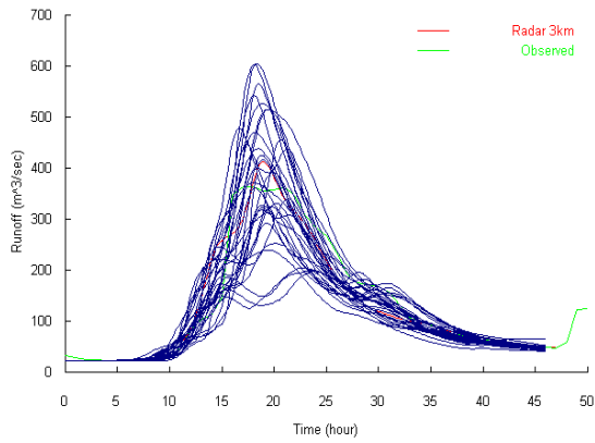
Fig. 16. Hydrographs at Ieno (476 km 2 ) obtained from the use of rainfall disaggregated by the RC method
