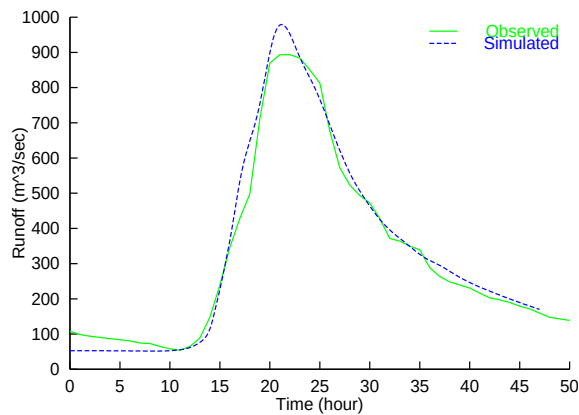
Fig. 7. Hydrograph at Kamo (1,469 km 2 )
