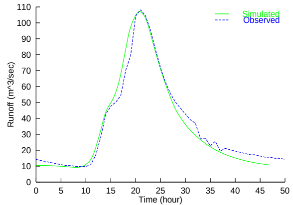
Fig. 9. Hydrograph at Ootori (156 km 2 )
