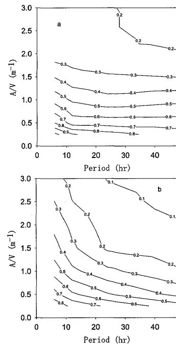
Figs. a and b : C-value contour diagrams of each period and A/V for porous ceramics (a) and sugi(b)
