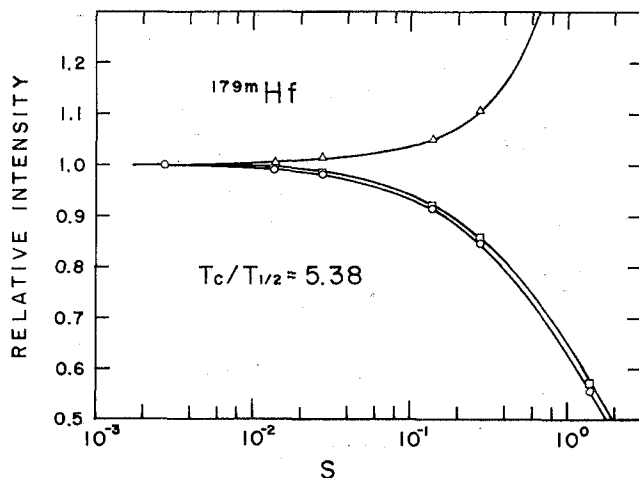
Fig. 5. Same as Fig. 2, but for ^{179\text{m}}\text{Hf} and for T_C=100 sec.
