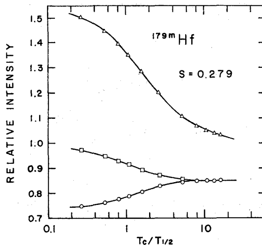
Fig. 6. Relative photopeak intensities for ^{179m}\text{Hf} as a function of the reduced measuring period T_c/T_{1/2} . The source intensity is 100\text{ }\mu\text{Ci} , which corresponds to S=0.279 .
