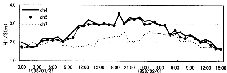
(a) Significant Wave Height(ch4,ch5.ch7)
