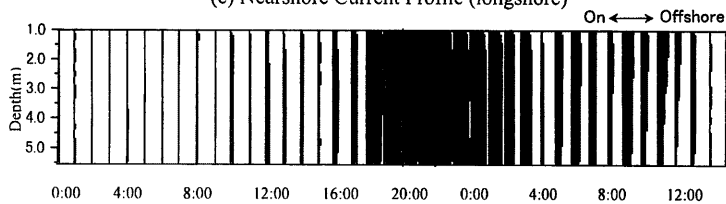
(c) Nearshore Current Profile (on-offshore)
