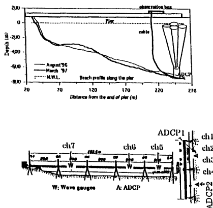
Figure1. Observation Pier and Equipment Set-up
