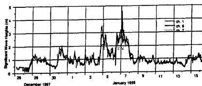
Figure2 Significant Wave Height (26th,Dec,1997 to 16th,Jan,1998)
