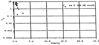
Figure9d Drag Coefficient Estimates against Wind Speed (tyre4)
