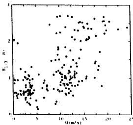
Figure11 Significant Wave Height against Wind Speed (tyre1)
