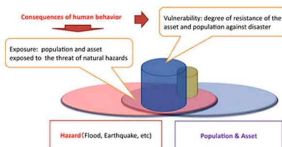
Fig. 3 Relationship between hazard, exposure and vulnerability
