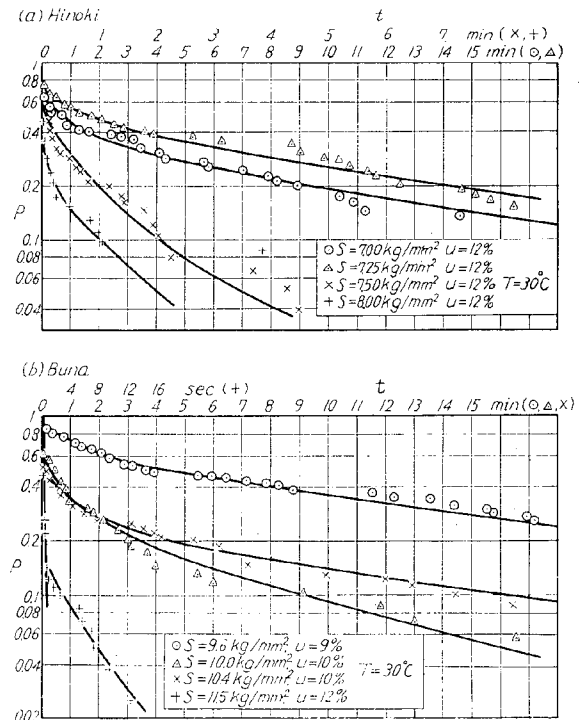
Fig. 9. Log P-t diagram—the effect of applied stress in dry condition.
