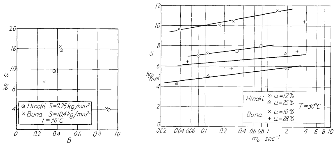
Fig. 15. Relation between moisture content and B in eq. (9).
