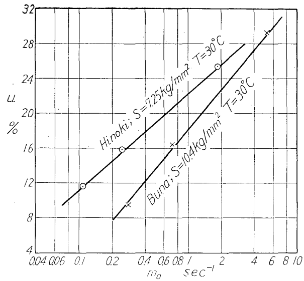
Fig. 13. Relation between moisture content and m_0 in eq. (11).
