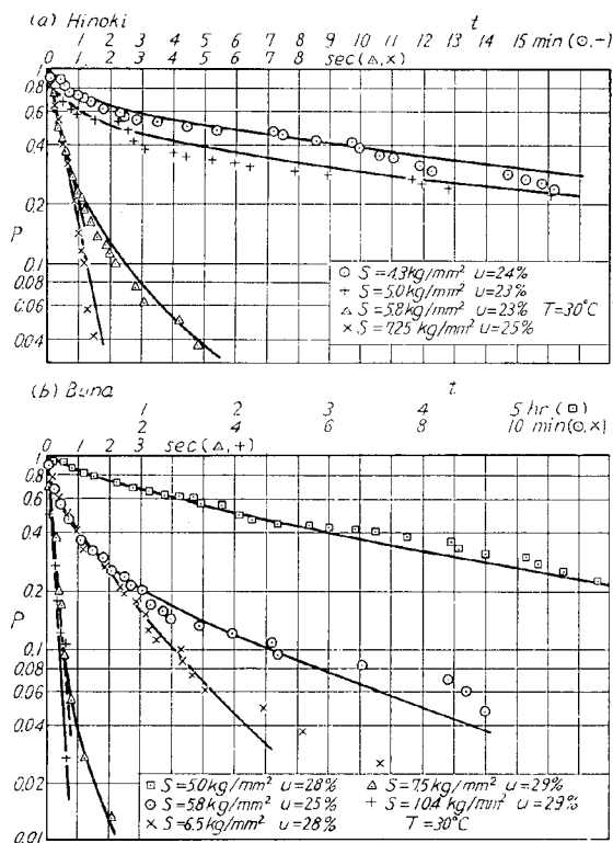
Fig. 10. Log P-t diagram—the effect of applied stress in wet condition.
