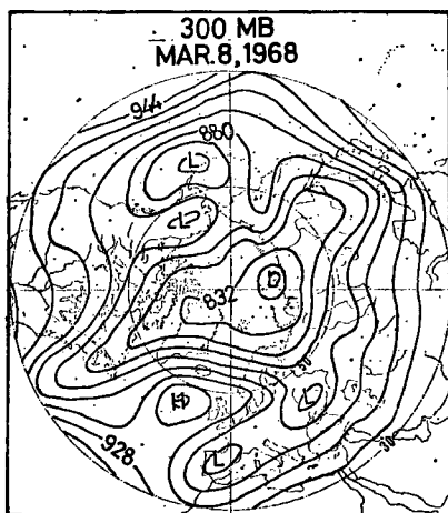
Fig. 3 300-mb contours in decameters for March 8, 1968.
