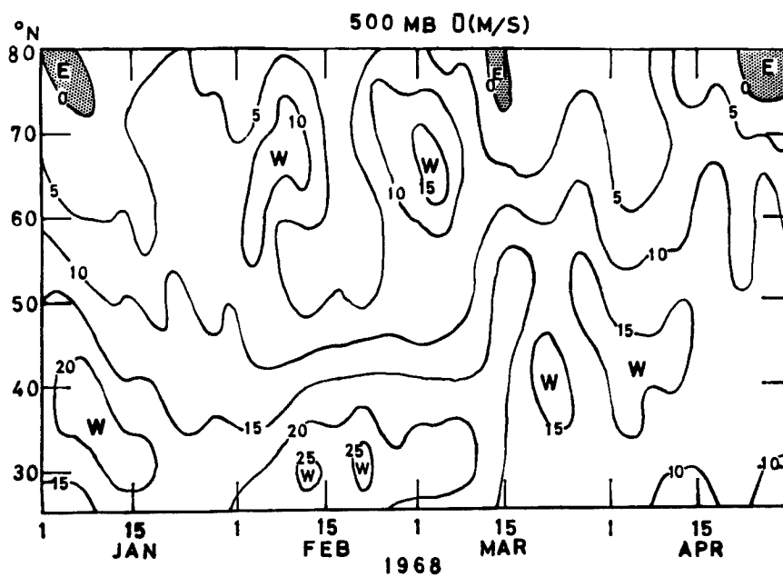
Fig. 4 Zonal mean wind in meters per second at 500-mb level for 1 January–30 April 1968.
