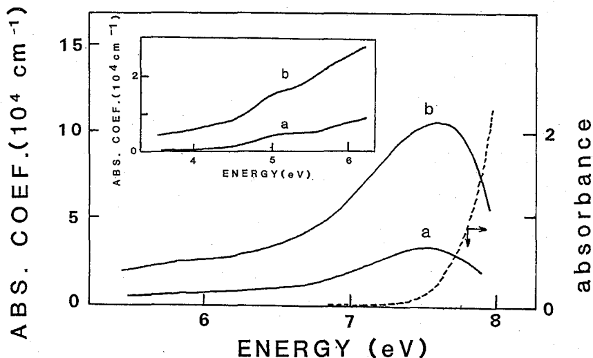
Fig. 1. Vacuum uv and uv absorptions induced by ion implantation. (a) \text{Cr } 0.5 \times 10^{16} ions/ \text{cm}^2 , (b) \text{Cr } 3 \times 10^{16} ions/ \text{cm}^2 . The dashed trace is the absorption spectrum of unimplanted substrate. The thickness of implanted layers are assumed to be 140 nm.
