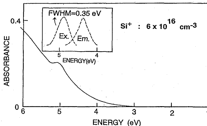
Fig. 7. Uv absorption spectrum of the substrate implanted with Si ion to dose of 6 \times 10^{16} \text{ ions/cm}^2 . The inset are emission and excitation spectra.
