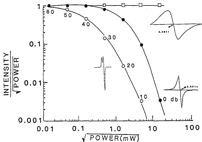
Fig. 3. Comparison of Microwave power saturation behavior among standard E' center ( \circ ), E' center ( \bullet ) produced by implantation, and E' type center ( \square ) associated with Si-Si bond.
