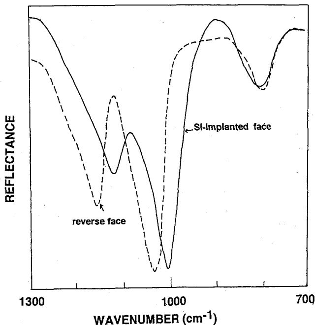
Fig. 5. FT-IR ATR spectra. —, Si 6 \times 10^{16} ions/ \text{cm}^2 implanted; ---; unimplanted face.
