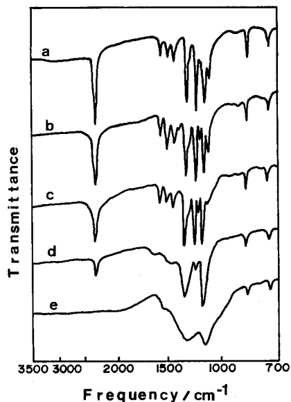
Fig. 2. IR spectra of films produced on copper film at 300°C (a), 350°C (b), 400°C (c), 450°C (d) and 500°C (e).
