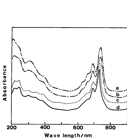
Fig. 1. UV/VIS spectra (in concd sulfuric acid) of films produced on copper film at 300°C (a), 350°C (b), 400°C (c) and 450°C (d).
