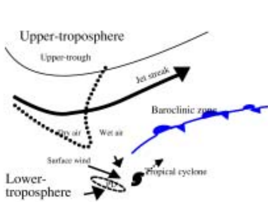
Fig.4 : Schematic illustration of the a statistical model of the PD.
