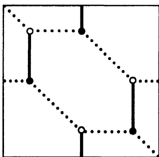
図 38: (h_x, h_y) = (1, 0)
