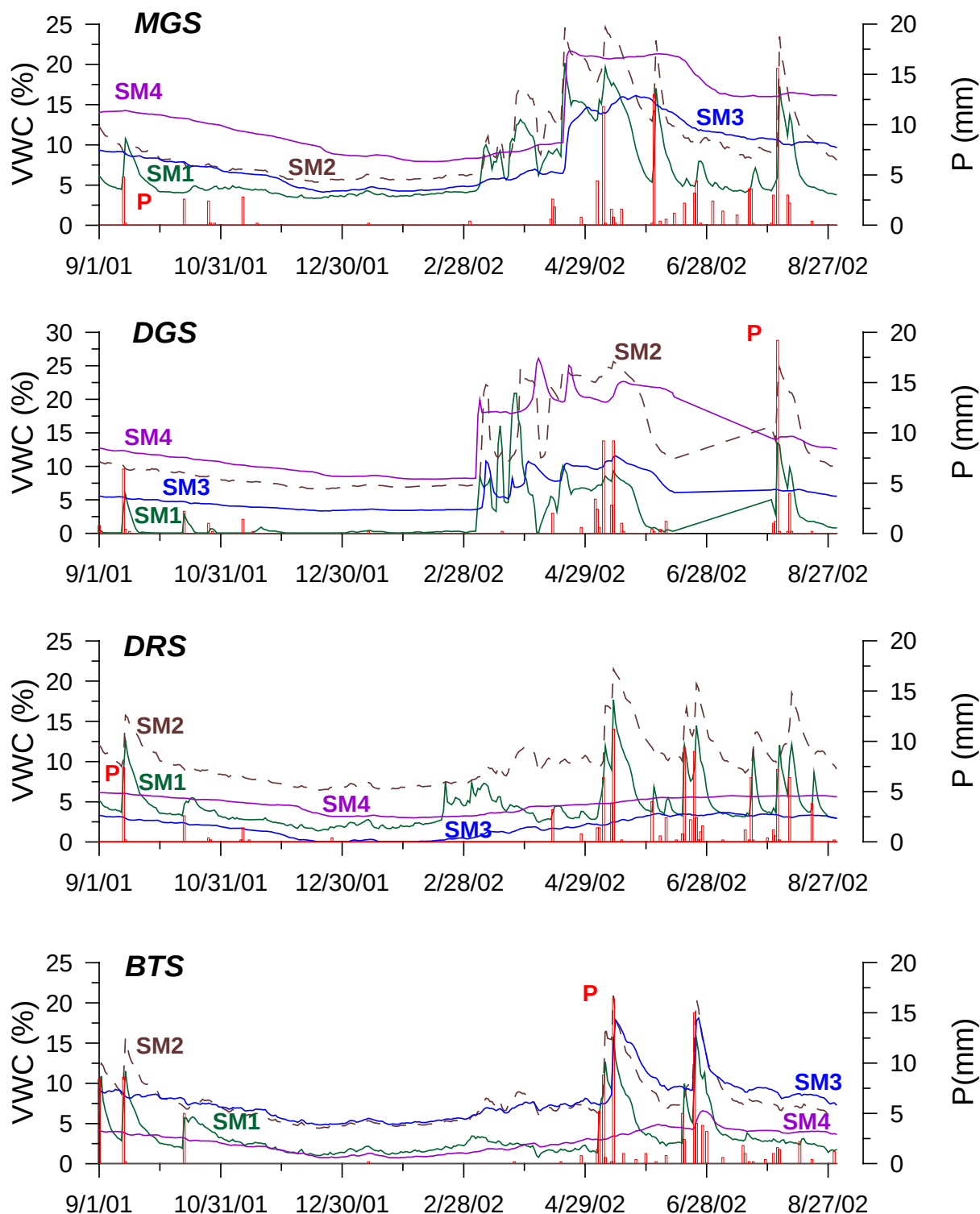
Fig. 1 Monitoring results of AWS at four sites (P: precipitation, VWC: volumetric water content of soil moisture) from Sep. 2001 to Aug. 2002 at BTS, DGS, MGS and DRS of AWS [Ts: surface soil temperature, Ta: air temperature, ST: soil temperature, 1: 3 cm depth, 2: 10 cm depth, 3: 40 cm depth, 4: 100 cm depth]
