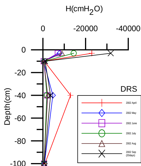
Fig. 3 Monthly mean total head profiles of DRS from April to September in 2002
