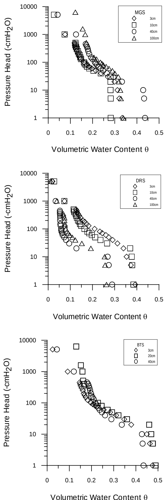
Fig. 2 Relationships between pressure head and volumetric water content of MGS, DRS and BTS soils
