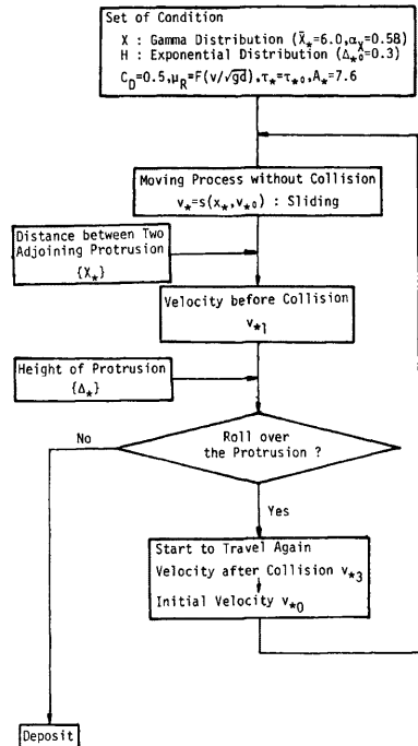
Fig. 29 Flow-chart for a numerical simulation.
