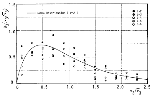
Fig. 18 Distribution of particle velocity after collision.
