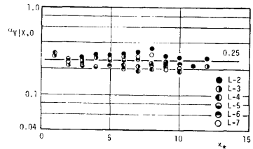
Fig. 25 Variation coefficient of particle velocity from incipient motion to the first collision.
