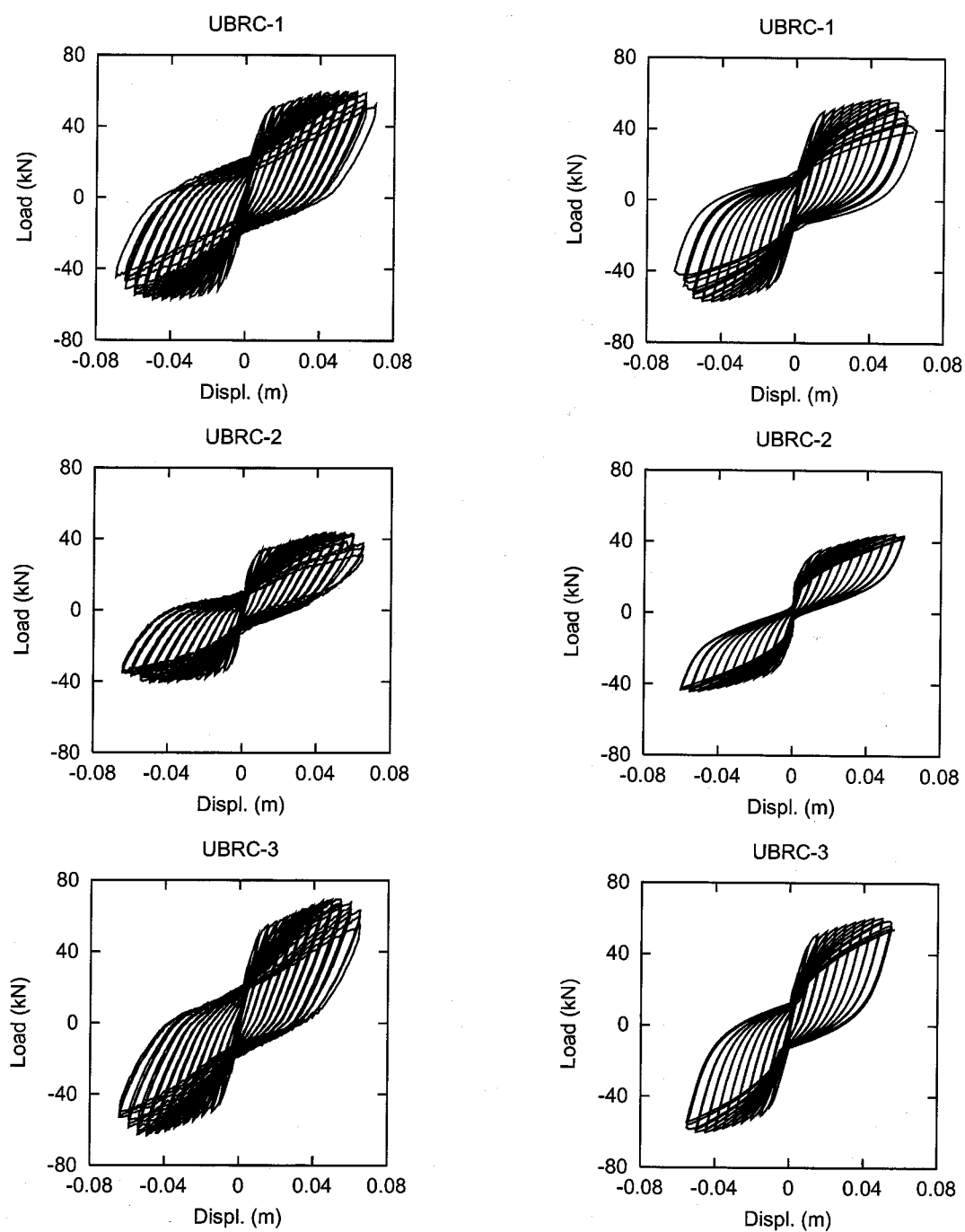
Figure 4.19: Comparison of Load–Displacement Hysteresis Loops
