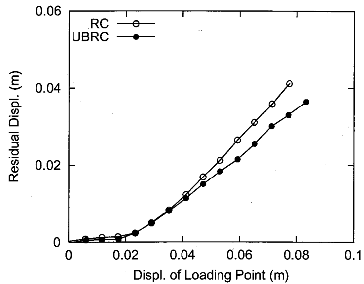
Figure 5.10: Residual Displacement
