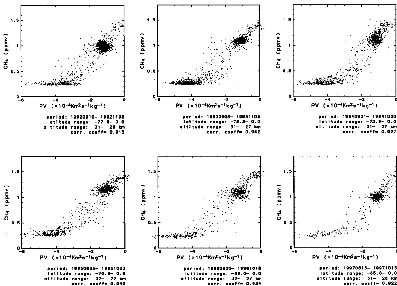
Figure 4. Plots of \text{CH}_4 versus PV on the 750-K isentropic surface for the six springs.
