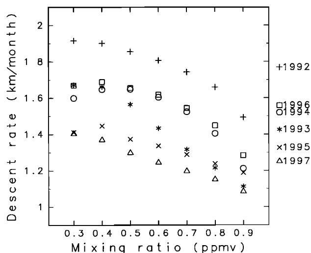
Figure 7. Average winter descent rates from fall to spring for each mixing ratio (0.3–0.9 ppmv). Values on the right axis are averages from 0.3 to 0.9 ppmv. Error bars (at 0.6 ppmv) for each year are indicated in Figure 9, because they have almost the same values in the range of 0.3–0.9 ppmv.
