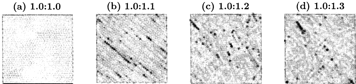
Figure 3: Snapshots of local stress. The shear field is applied horizontally: (a)(pure crystal) is already ruptured.
