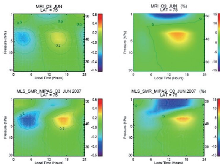
Figure Local time-pressure cross sections of zonal-mean ozone diurnal variation fields (in ppmv) in June 2007 at 75^\circ N (left) and percent deviations (right) from the midnight values at each pressure level. The data are derived from the MRI-CCM simulation (top) and from the combined MLS/Aura, SMR/Odin, and MIPAS/Envisat measurements in 2007 (bottom). 0 h is midnight, and 12 h is noon.
