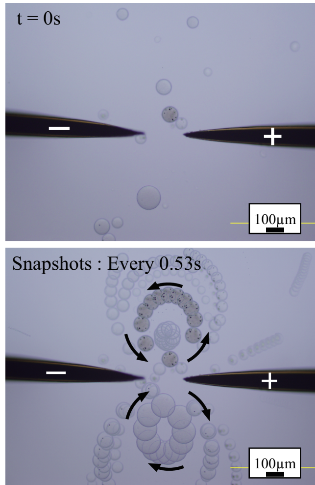
FIGURE 5.2: Self-revolution of plastic particles. (a) Initial condition at t=0\text{ s} from when DC voltage is applied. (b) Overlap of snapshots at every 0.53\text{ s} . Plural number of polystyrene particles with the radii of r = 50 - 175\mu\text{m} are rotating in the oil phase with anionic surfactant at V=170\text{ V} .
