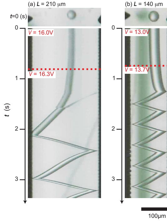
FIGURE 3.3: Spatio-temporal diagram of the motion of a droplet with a diameter of 34\mu\text{m} at (a) L = 210\mu\text{m} and (b) L = 140\mu\text{m} . An increase in the applied DC voltage results in bifurcation from the static stationary to an oscillatory state.
