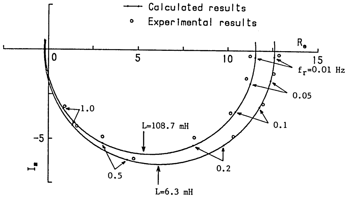
Fig.2.24. Frequency responses for G=20.9 \text{ mS} , K_b=0 , \alpha=80^\circ and e_I=2.6 \text{ V} .
