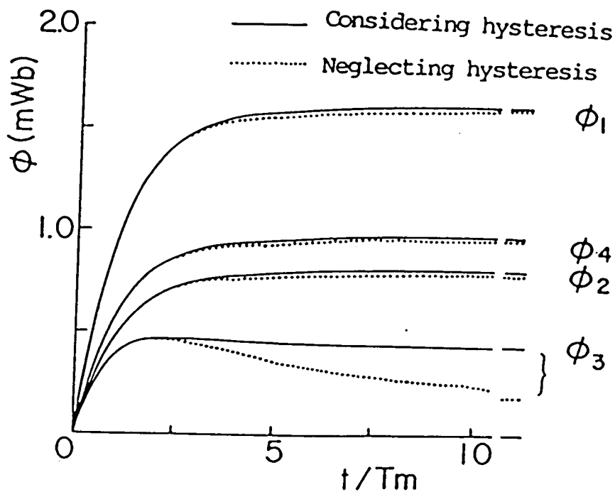
Fig.3.19 Influence of magnetic hysteresis on transient responses of magnetic fluxes.
