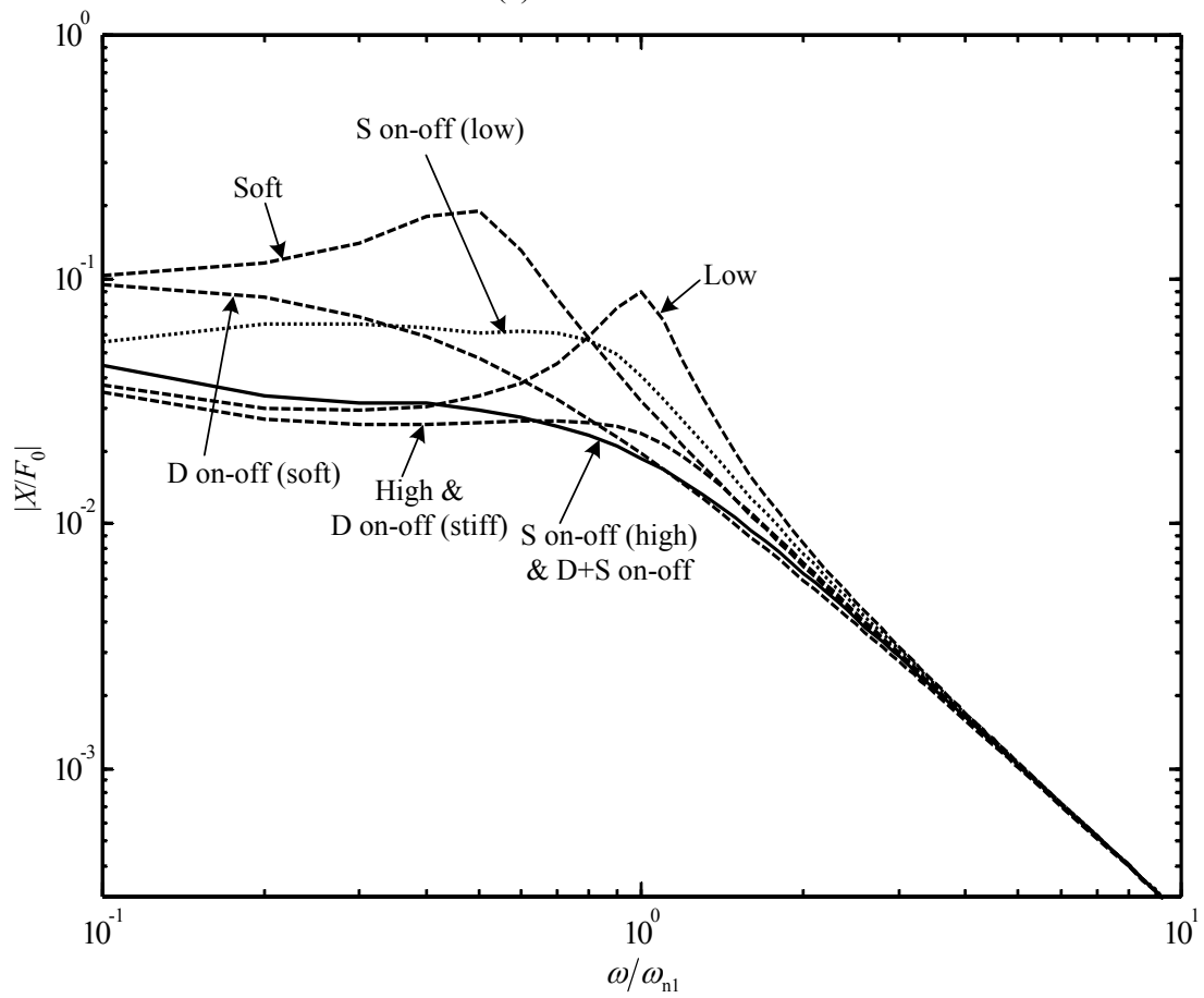
Fig. 5 Frequency responses of the system to a sinusoidal excitation.
