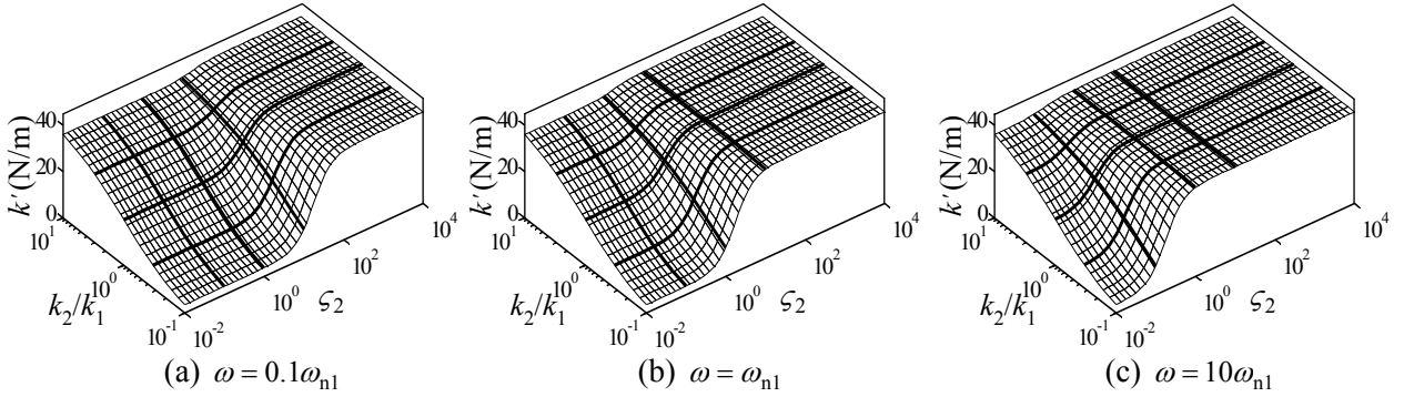
Fig. 3 Equivalent stiffness of the system.
