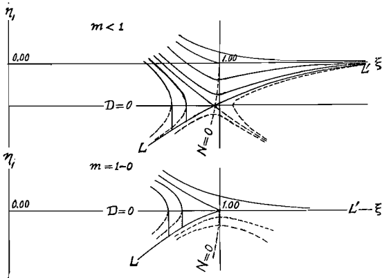
Fig. 5. Possible forms of attendant water surface at the forward end of the disturbance; m \leq 1 .
