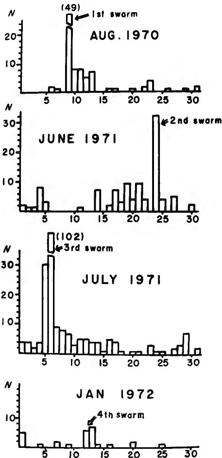
Fig. 2. Daily sums of number of earthquakes recorded at LAB for a month within which the swarm occurred.
