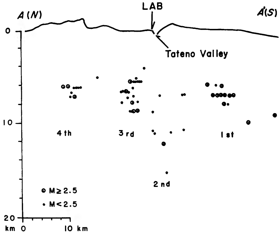
Fig. 6. Distribution of foci on a cross section AA' in Fig. 5 for all swarms.
