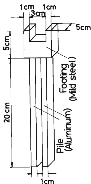
Fig. 3 Detail of the pile foundation
