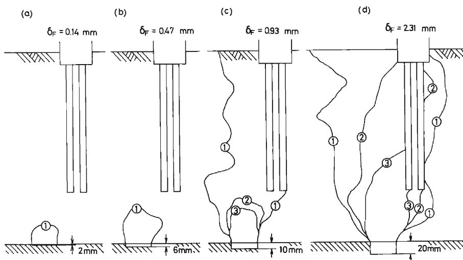
Fig. 13 Development of the equi-settlement contour lines for H=30\text{ cm} and e=5\text{ cm}
