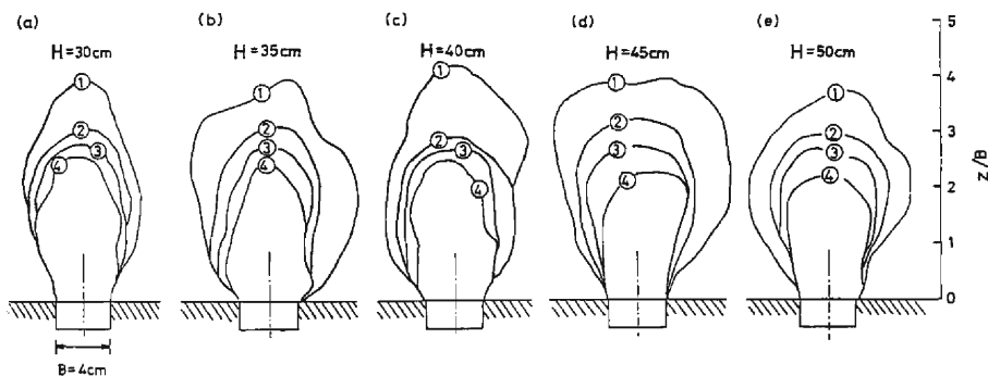
Fig. 12 Equi-settlement contour lines at \delta_L=20\text{ mm}
