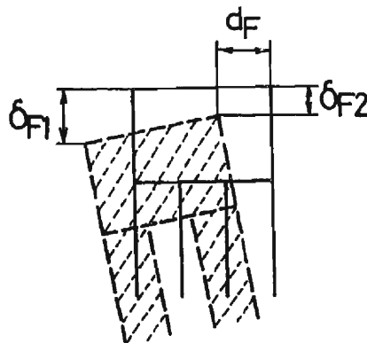
Fig. 5 Displacement of the pile footing
