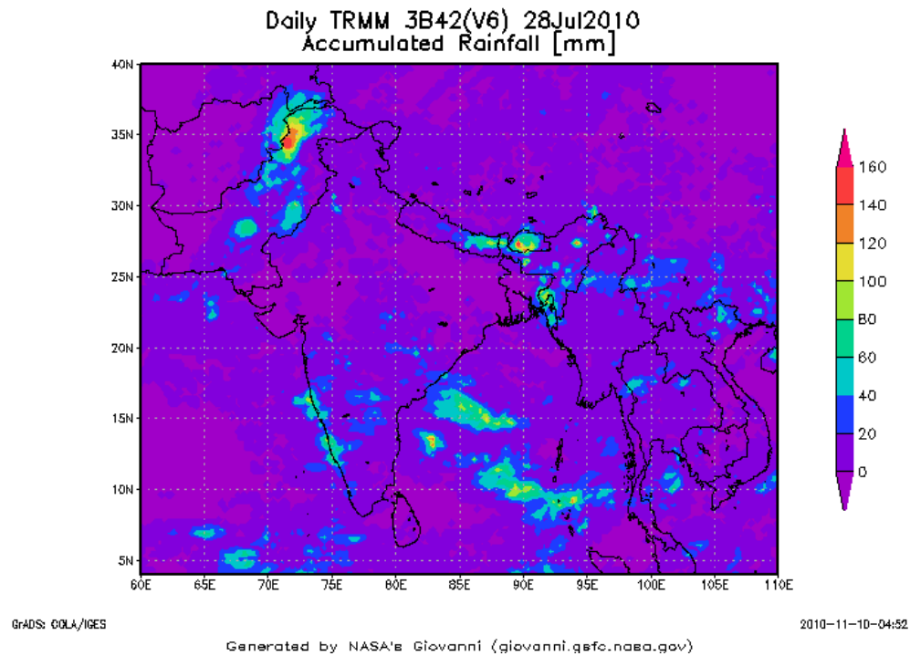
Figure 2.4 Daily TRMM 3B42_V6 rainfall estimates in the South Asia domain
