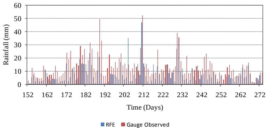
Figure 3.25 Daily basin averaged gauge observed rainfall with RFE for JJAS of 2003 in the Narayani Basin
