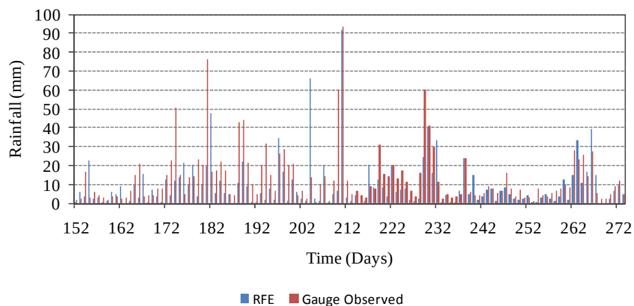
Figure 3.22 Daily basin averaged gauge observed rainfall with RFE for JJAS of 2003 in the Bagmati Basin
