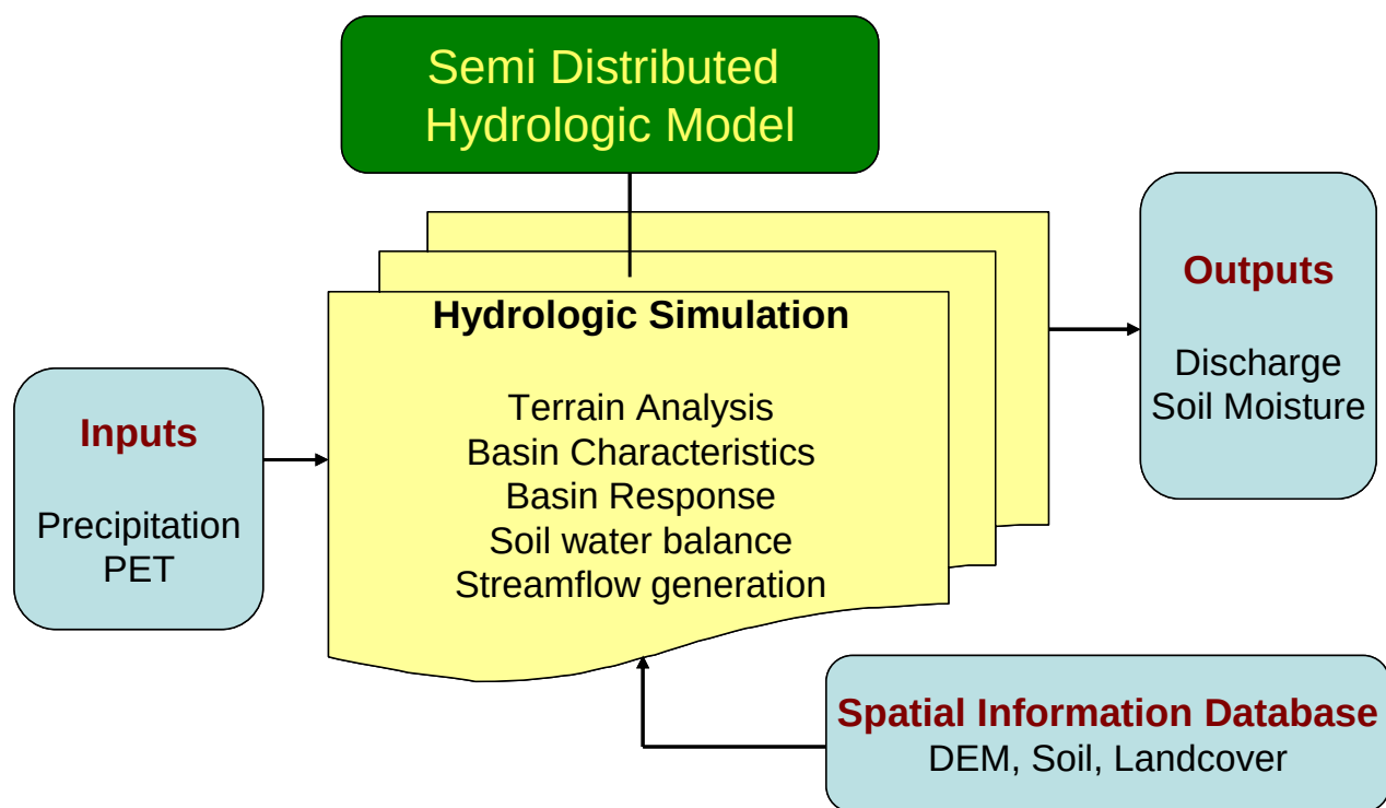
Figure 4.1 General framework of the GeoSFM model
