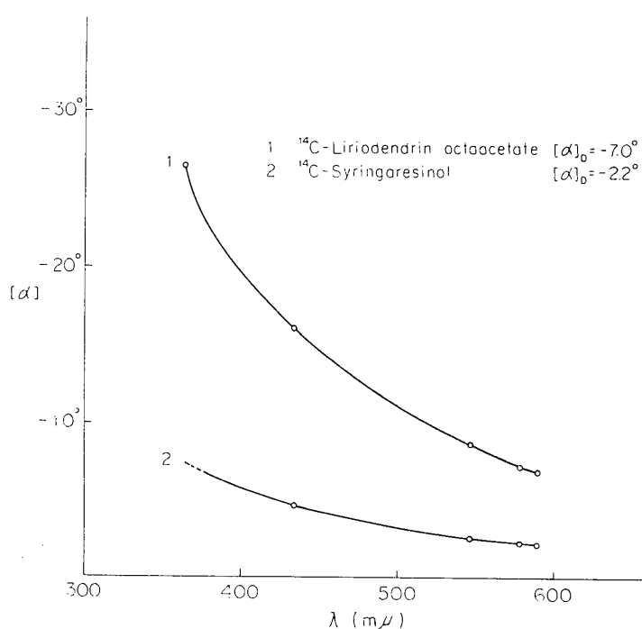
Fig. 3. Optical rotation of ^{14} C-liriodendrin octaacetate and ^{14} C-syringaresinol.
