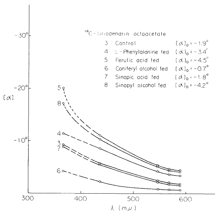
Fig. 4. Optical rotation of ^{14}\text{C} -liriodendrin octaacetate.
