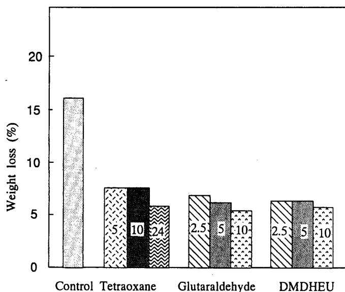
Fig. 4. The weight loss of cross-linking agents-treated LVLs after 9 week exposure to termite.
