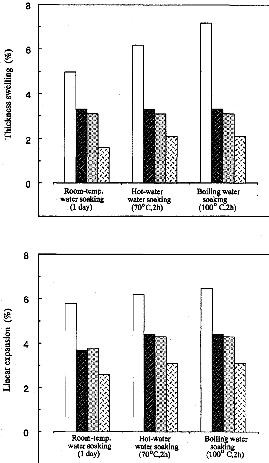
Fig. 7. Thickness swelling and linear expansion of DMDHEU-treated after water immersion. Legend: See Fig. 6.
