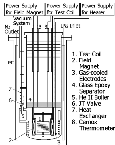
Fig. 1. Experimental apparatus.
